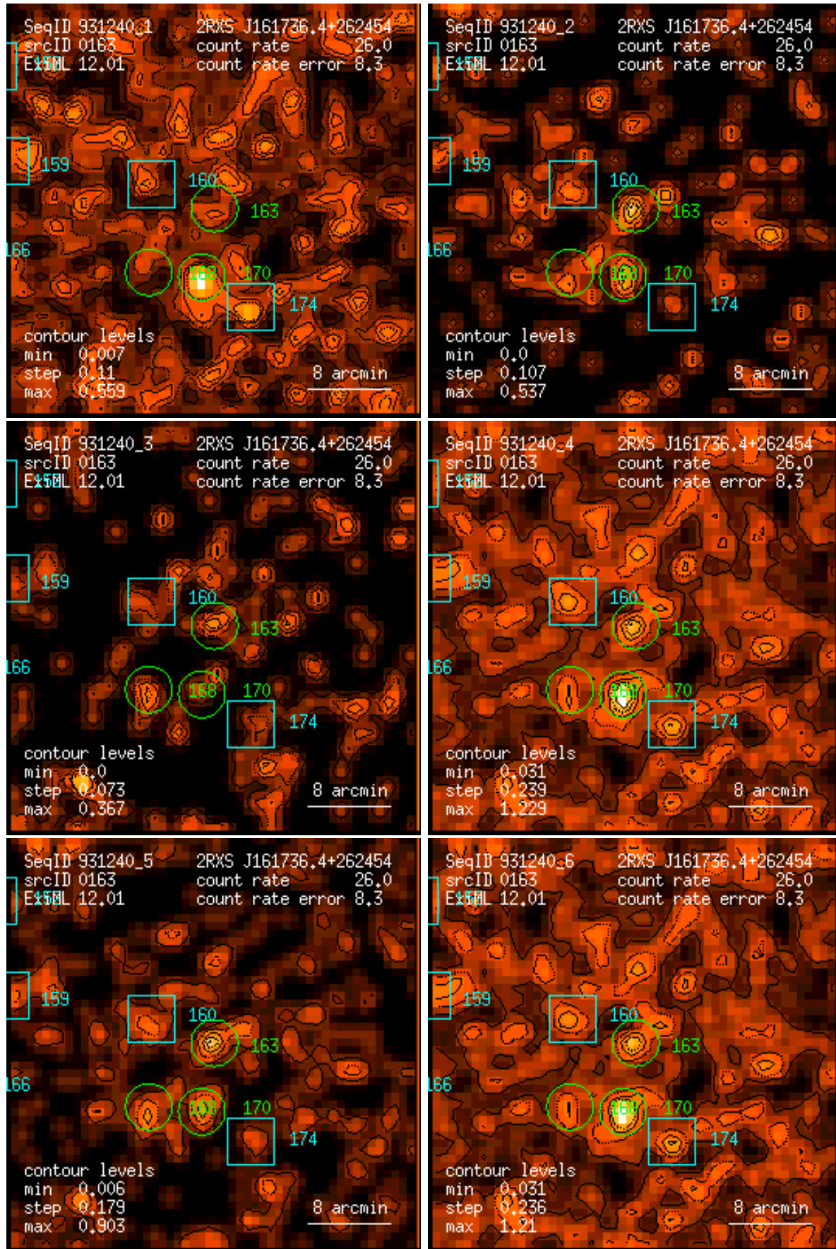
Figure 163: RASS 931240: detection 0163: band rate images, Gaussian filter: (1) PSPC channels 11 – 41, (2) 52 – 90, (3) 91 – 201, (4) 11 – 235, (5) 52 – 201, (6) 11 – 201. Broad band rates in counts/ks. Band rate contour levels in counts/ks/arcmin 2 .
