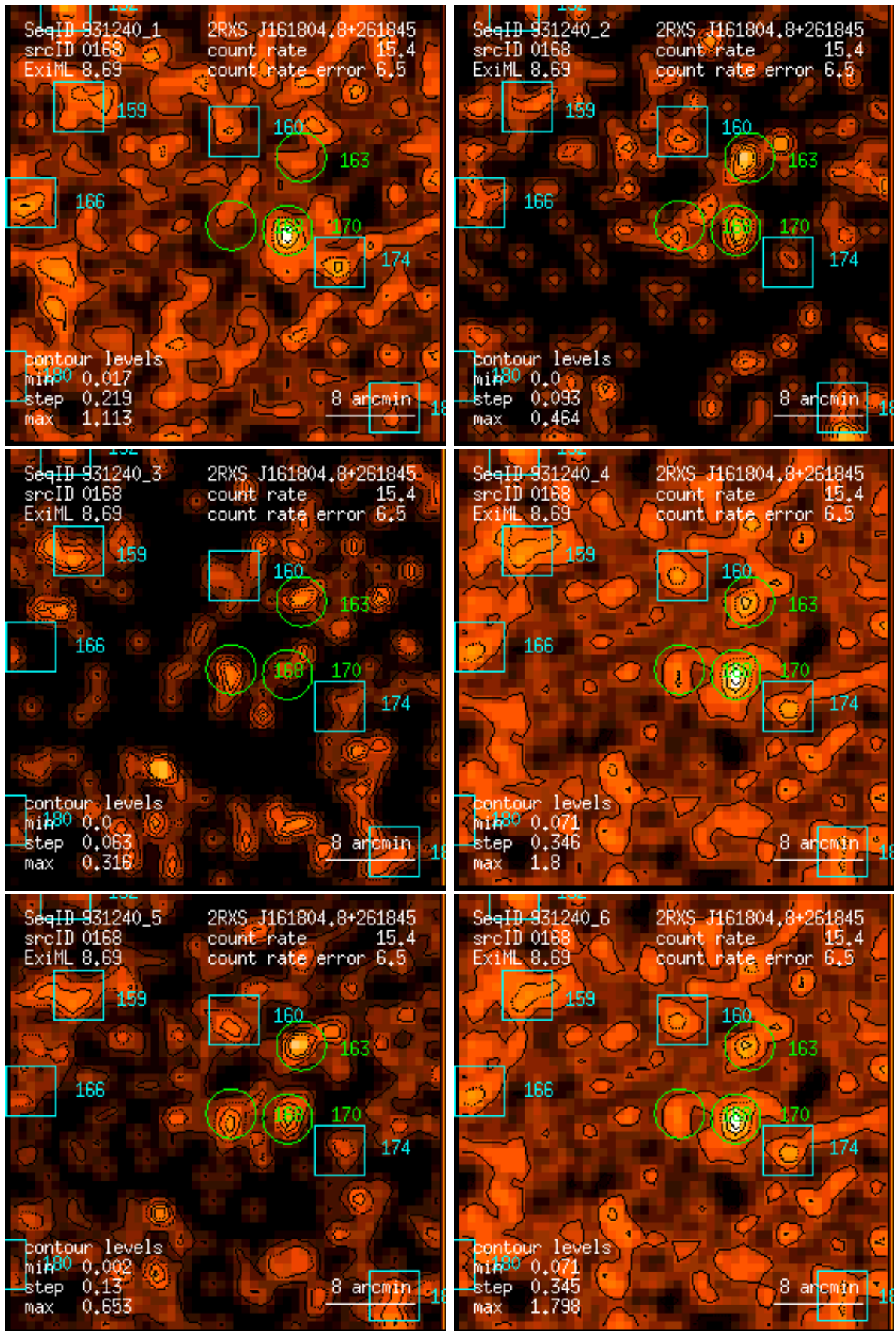
Figure 168: RASS 931240: detection 0168: band rate images, Gaussian filter: (1) PSPC channels 11 – 41, (2) 52 – 90, (3) 91 – 201, (4) 11 – 235, (5) 52 – 201, (6) 11 – 201. Broad band rates in counts/ks. Band rate contour levels in counts/ks/arcmin 2 .
