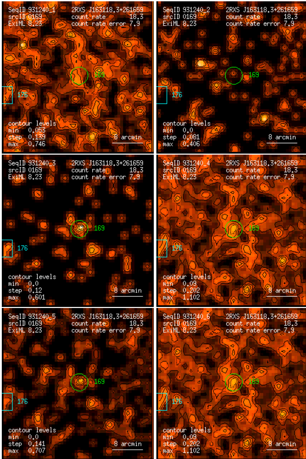
Figure 169: RASS 931240: detection 0169: band rate images, Gaussian filter: (1) PSPC channels 11 – 41, (2) 52 – 90, (3) 91 – 201, (4) 11 – 235, (5) 52 – 201, (6) 11 – 201. Broad band rates in counts/ks. Band rate contour levels in counts/ks/arcmin 2 .
