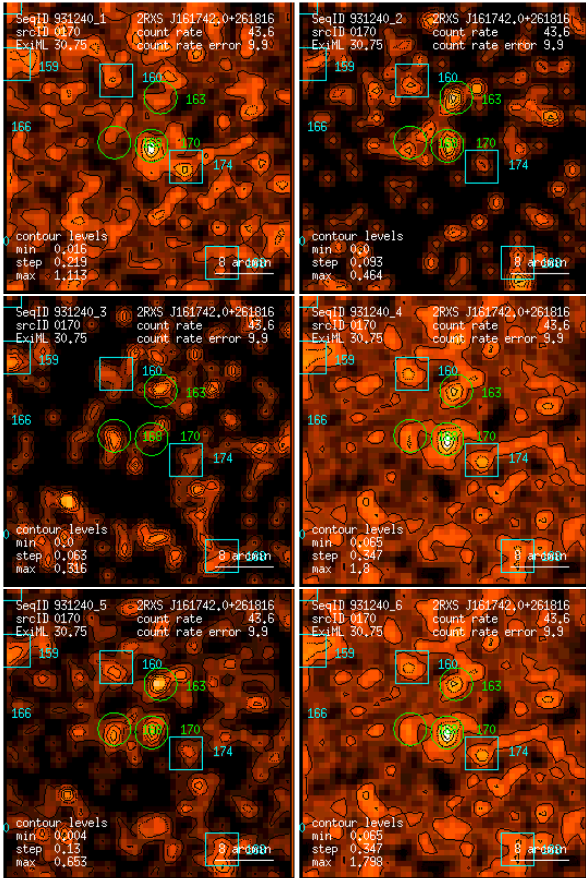
Figure 170: RASS 931240: detection 0170: band rate images, Gaussian filter: (1) PSPC channels 11 – 41, (2) 52 – 90, (3) 91 – 201, (4) 11 – 235, (5) 52 – 201, (6) 11 – 201. Broad band rates in counts/ks. Band rate contour levels in counts/ks/arcmin 2 .
