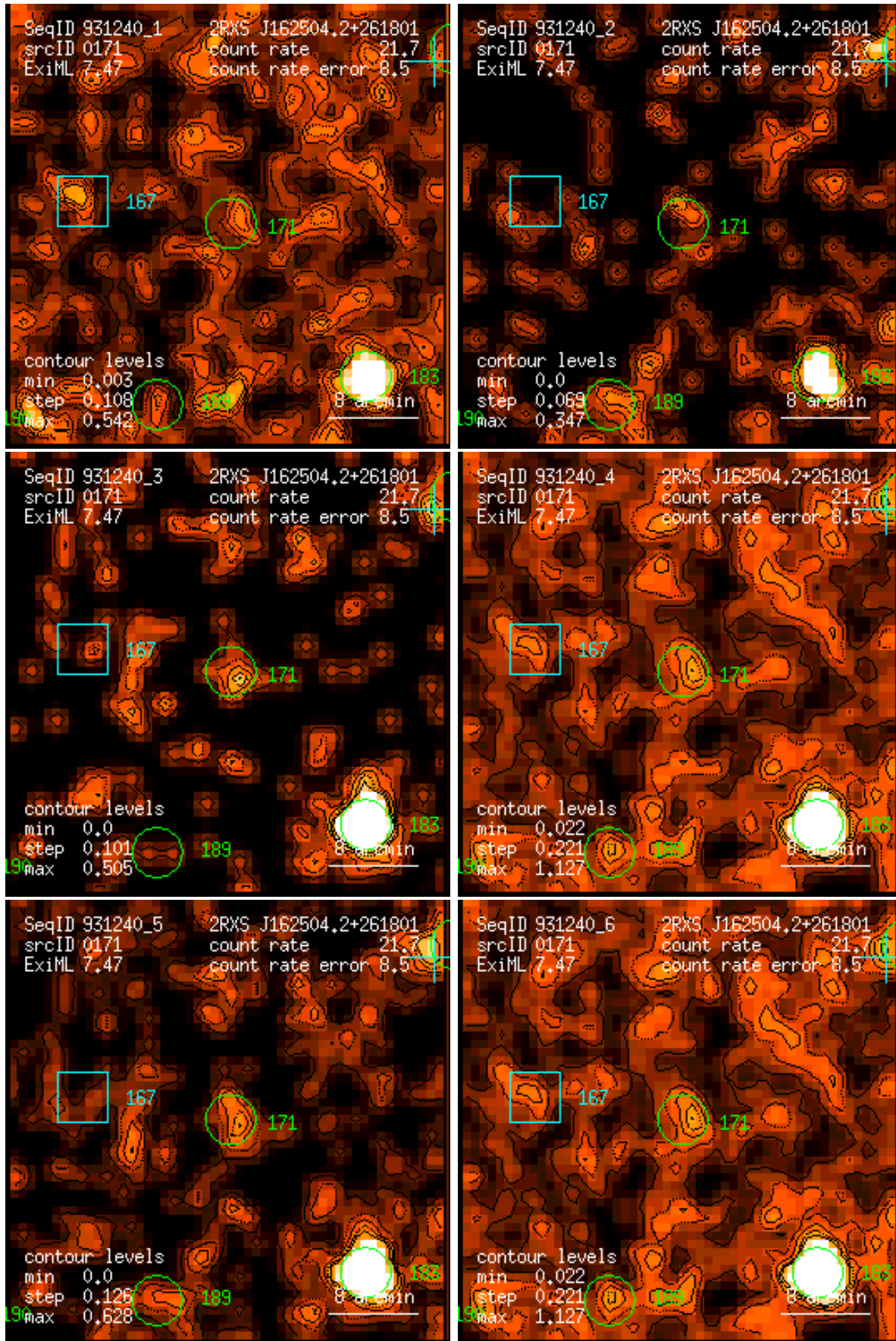
Figure 171: RASS 931240: detection 0171: band rate images, Gaussian filter: (1) PSPC channels 11 – 41, (2) 52 – 90, (3) 91 – 201, (4) 11 – 235, (5) 52 – 201, (6) 11 – 201. Broad band rates in counts/ks. Band rate contour levels in counts/ks/arcmin 2 .
