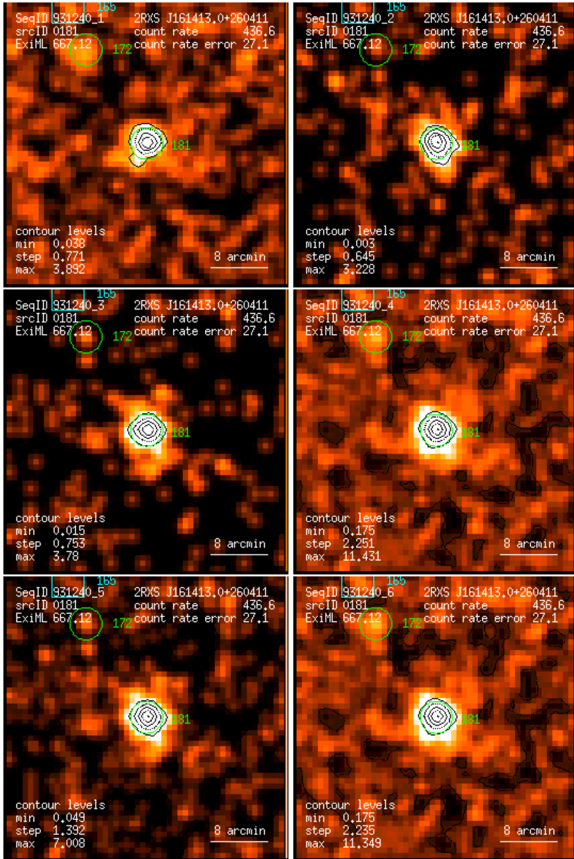
Figure 181: RASS 931240: detection 0181: band rate images, Gaussian filter: (1) PSPC channels 11 – 41, (2) 52 – 90, (3) 91 – 201, (4) 11 – 235, (5) 52 – 201, (6) 11 – 201. Broad band rates in counts/ks. Band rate contour levels in counts/ks/arcmin 2 .
