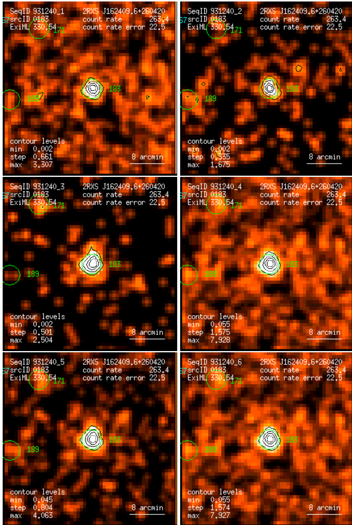
Figure 183: RASS 931240: detection 0183: band rate images, Gaussian filter: (1) PSPC channels 11 – 41, (2) 52 – 90, (3) 91 – 201, (4) 11 – 235, (5) 52 – 201, (6) 11 – 201. Broad band rates in counts/ks. Band rate contour levels in counts/ks/arcmin 2 .
