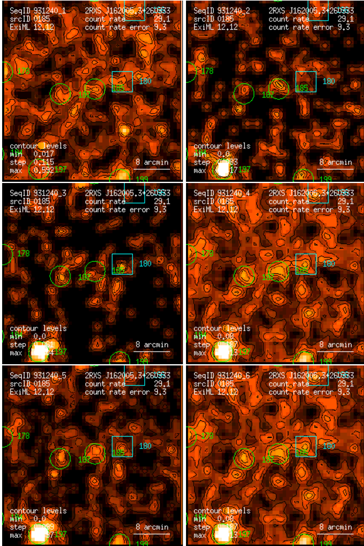
Figure 185: RASS 931240: detection 0185: band rate images, Gaussian filter: (1) PSPC channels 11 – 41, (2) 52 – 90, (3) 91 – 201, (4) 11 – 235, (5) 52 – 201, (6) 11 – 201. Broad band rates in counts/ks. Band rate contour levels in counts/ks/arcmin 2 .
