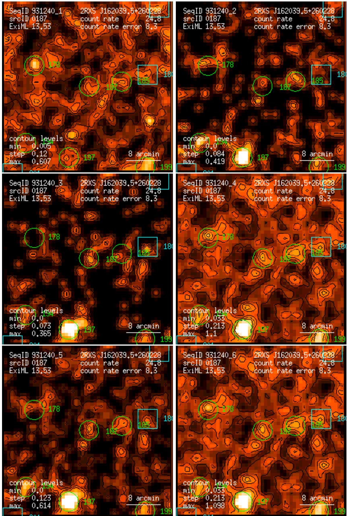
Figure 187: RASS 931240: detection 0187: band rate images, Gaussian filter: (1) PSPC channels 11 – 41, (2) 52 – 90, (3) 91 – 201, (4) 11 – 235, (5) 52 – 201, (6) 11 – 201. Broad band rates in counts/ks. Band rate contour levels in counts/ks/arcmin 2 .
