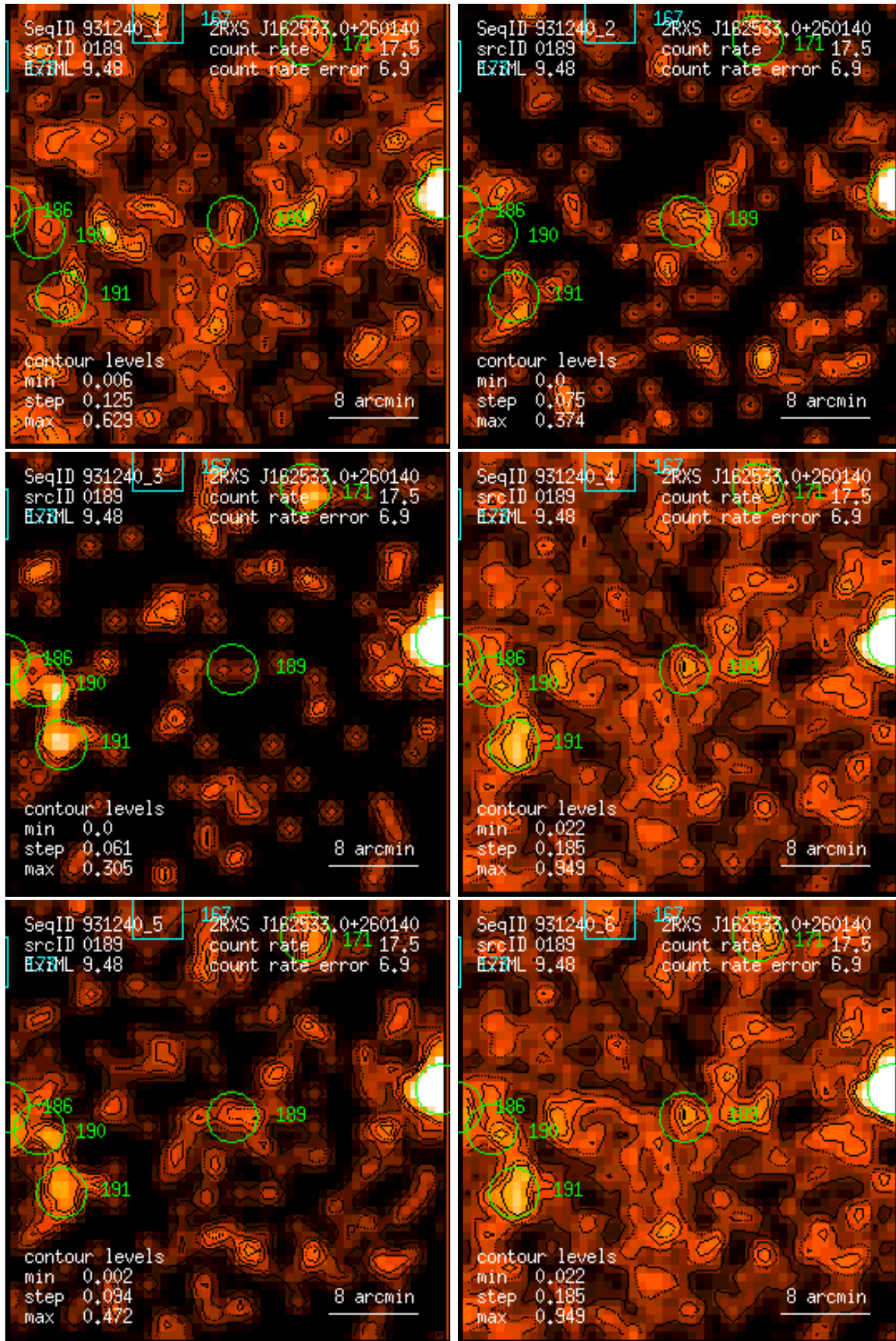
Figure 189: RASS 931240: detection 0189: band rate images, Gaussian filter: (1) PSPC channels 11 – 41, (2) 52 – 90, (3) 91 – 201, (4) 11 – 235, (5) 52 – 201, (6) 11 – 201. Broad band rates in counts/ks. Band rate contour levels in counts/ks/arcmin 2 .
