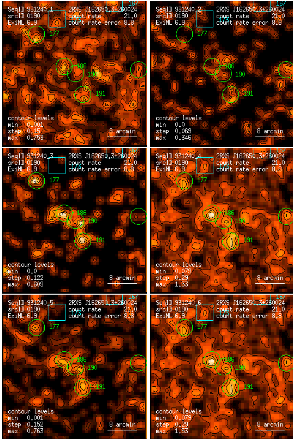
Figure 190: RASS 931240: detection 0190: band rate images, Gaussian filter: (1) PSPC channels 11 – 41, (2) 52 – 90, (3) 91 – 201, (4) 11 – 235, (5) 52 – 201, (6) 11 – 201. Broad band rates in counts/ks. Band rate contour levels in counts/ks/arcmin 2 .
