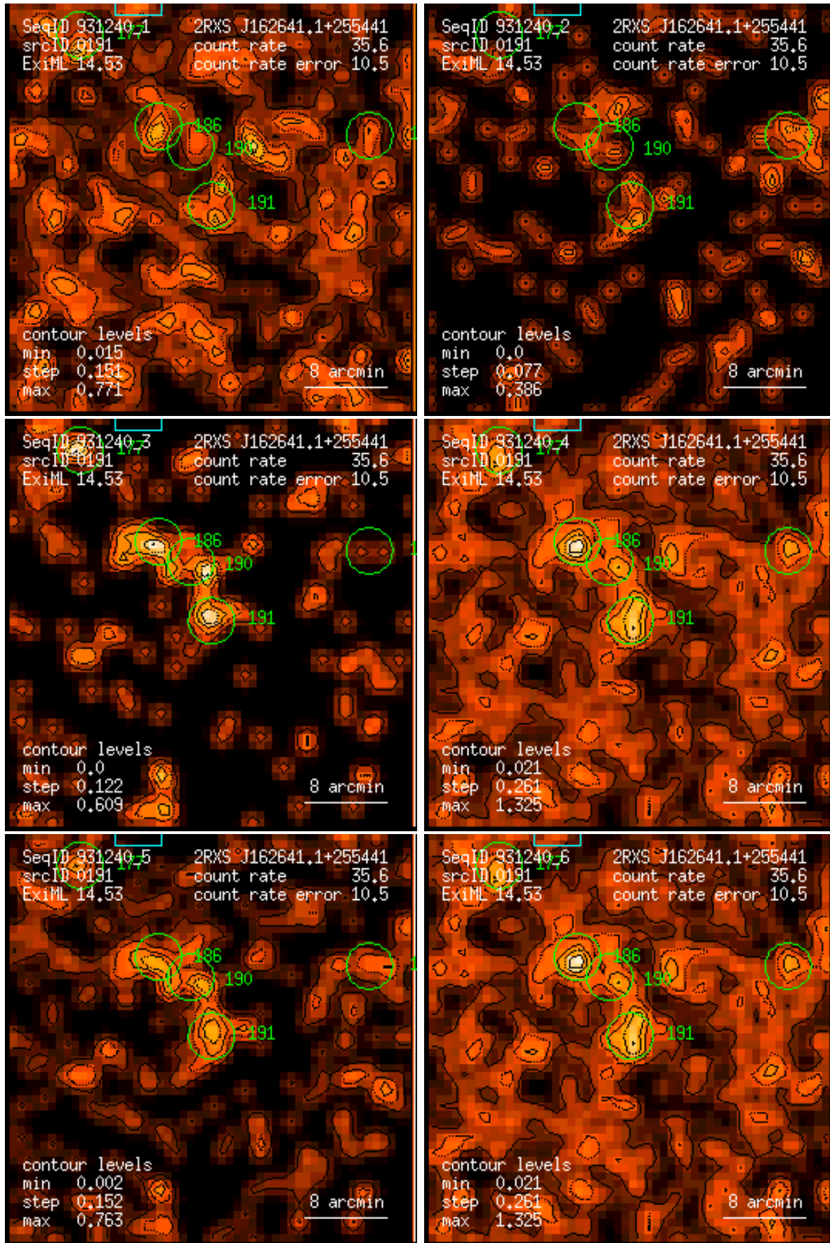
Figure 191: RASS 931240: detection 0191: band rate images, Gaussian filter: (1) PSPC channels 11 – 41, (2) 52 – 90, (3) 91 – 201, (4) 11 – 235, (5) 52 – 201, (6) 11 – 201. Broad band rates in counts/ks. Band rate contour levels in counts/ks/arcmin 2 .
