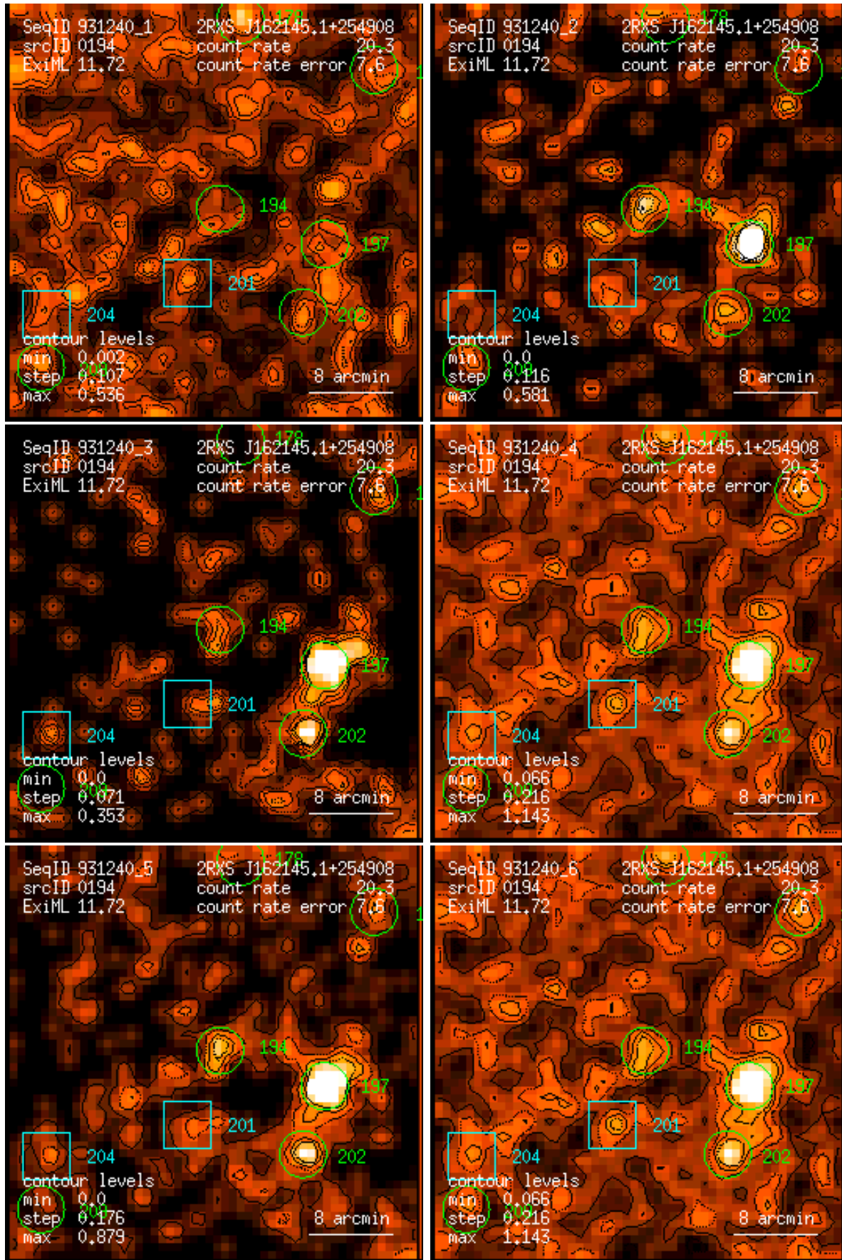
Figure 194: RASS 931240: detection 0194: band rate images, Gaussian filter: (1) PSPC channels 11 – 41, (2) 52 – 90, (3) 91 – 201, (4) 11 – 235, (5) 52 – 201, (6) 11 – 201. Broad band rates in counts/ks. Band rate contour levels in counts/ks/arcmin 2 .
