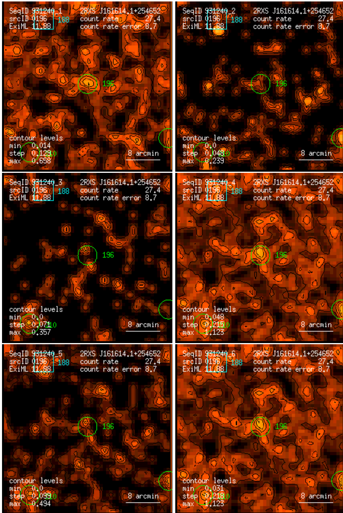
Figure 196: RASS 931240: detection 0196: band rate images, Gaussian filter: (1) PSPC channels 11 – 41, (2) 52 – 90, (3) 91 – 201, (4) 11 – 235, (5) 52 – 201, (6) 11 – 201. Broad band rates in counts/ks. Band rate contour levels in counts/ks/arcmin 2 .
