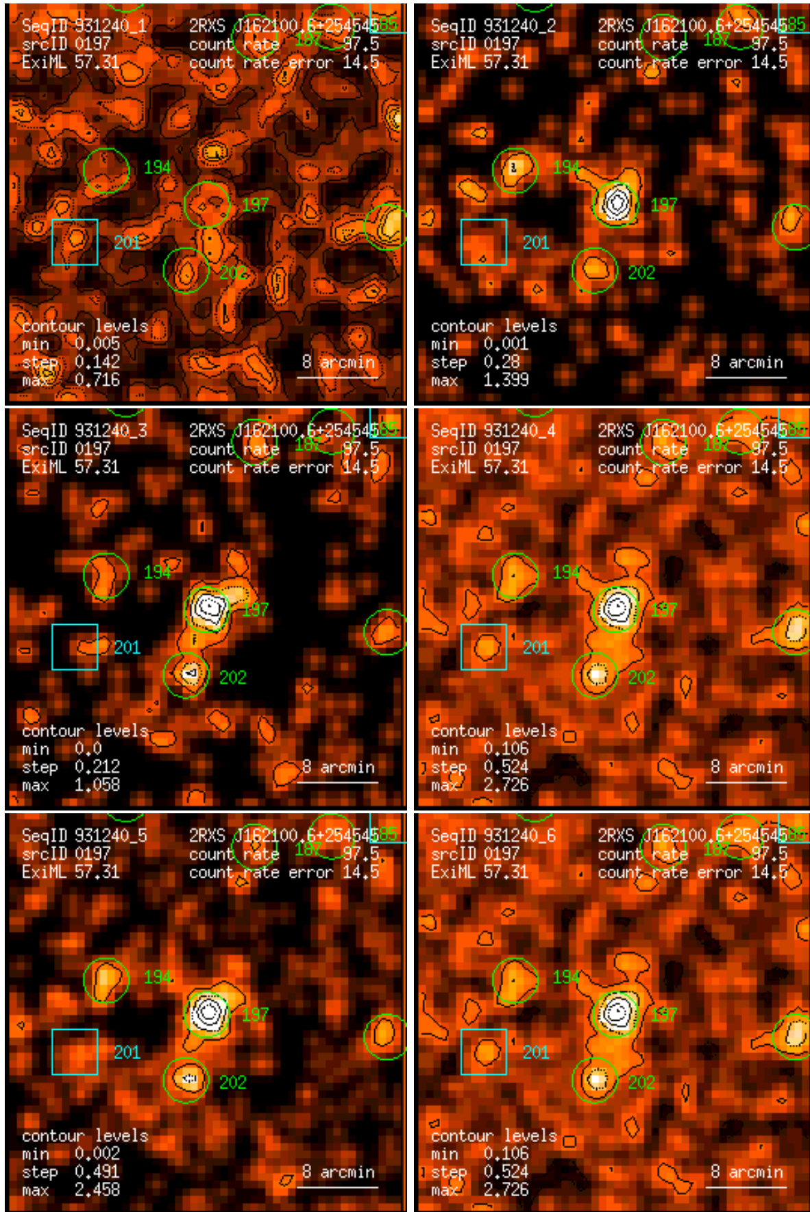
Figure 197: RASS 931240: detection 0197: band rate images, Gaussian filter: (1) PSPC channels 11 – 41, (2) 52 – 90, (3) 91 – 201, (4) 11 – 235, (5) 52 – 201, (6) 11 – 201. Broad band rates in counts/ks. Band rate contour levels in counts/ks/arcmin 2 .
