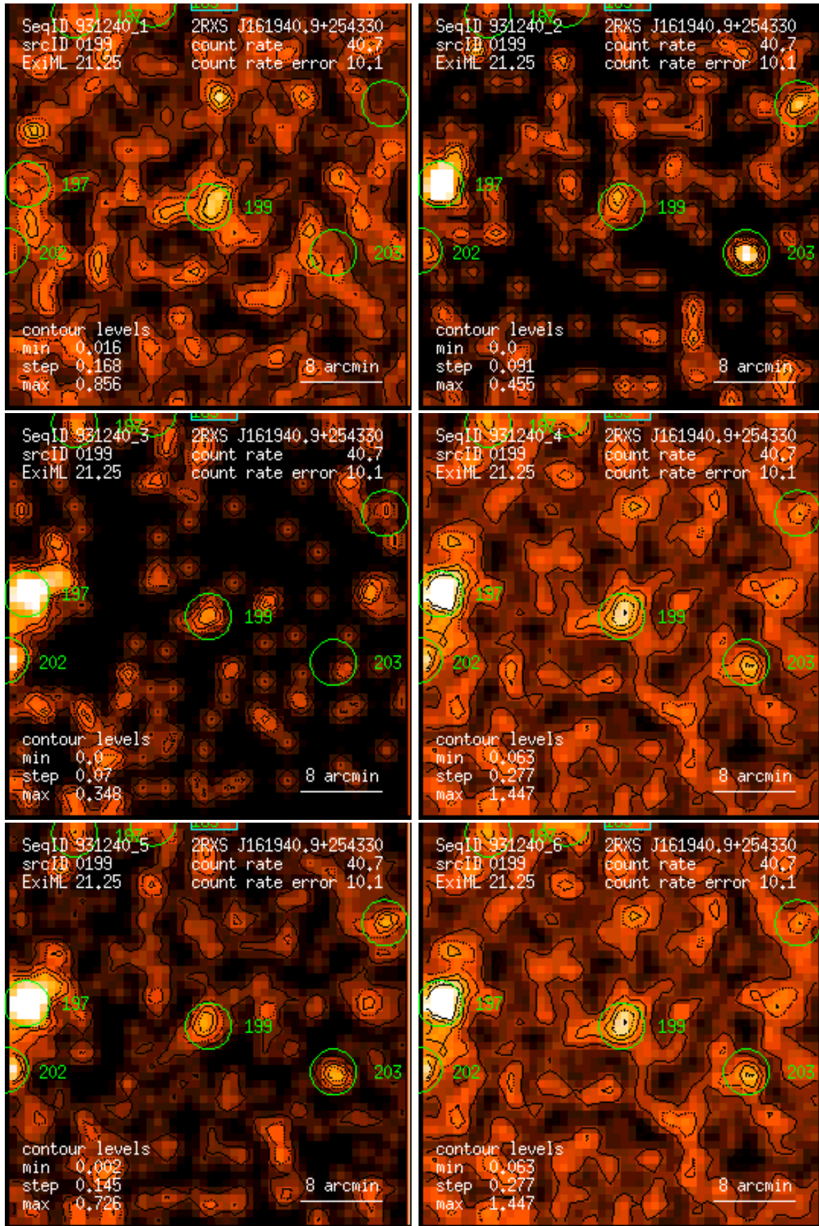
Figure 199: RASS 931240: detection 0199: band rate images, Gaussian filter: (1) PSPC channels 11 – 41, (2) 52 – 90, (3) 91 – 201, (4) 11 – 235, (5) 52 – 201, (6) 11 – 201. Broad band rates in counts/ks. Band rate contour levels in counts/ks/arcmin 2 .
