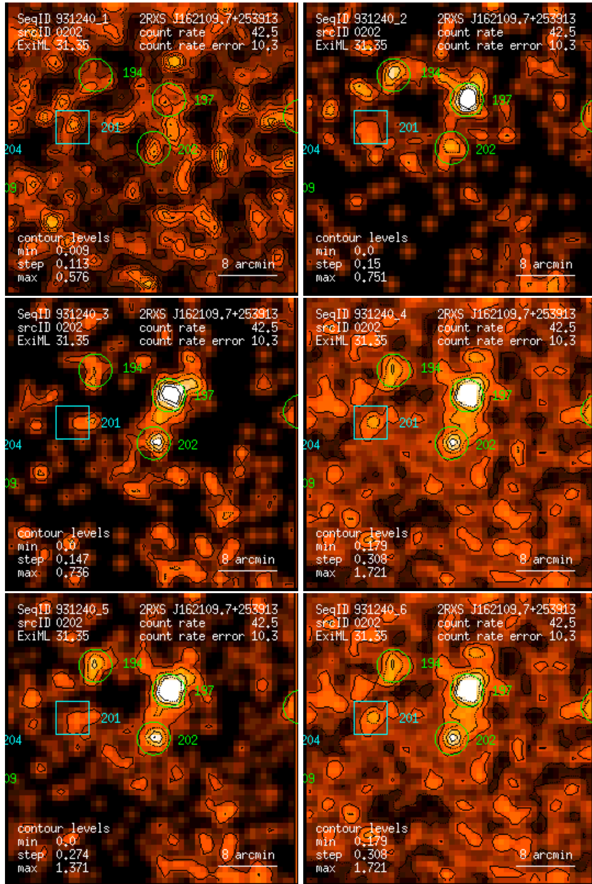
Figure 202: RASS 931240: detection 0202: band rate images, Gaussian filter: (1) PSPC channels 11 – 41, (2) 52 – 90, (3) 91 – 201, (4) 11 – 235, (5) 52 – 201, (6) 11 – 201. Broad band rates in counts/ks. Band rate contour levels in counts/ks/arcmin 2 .
