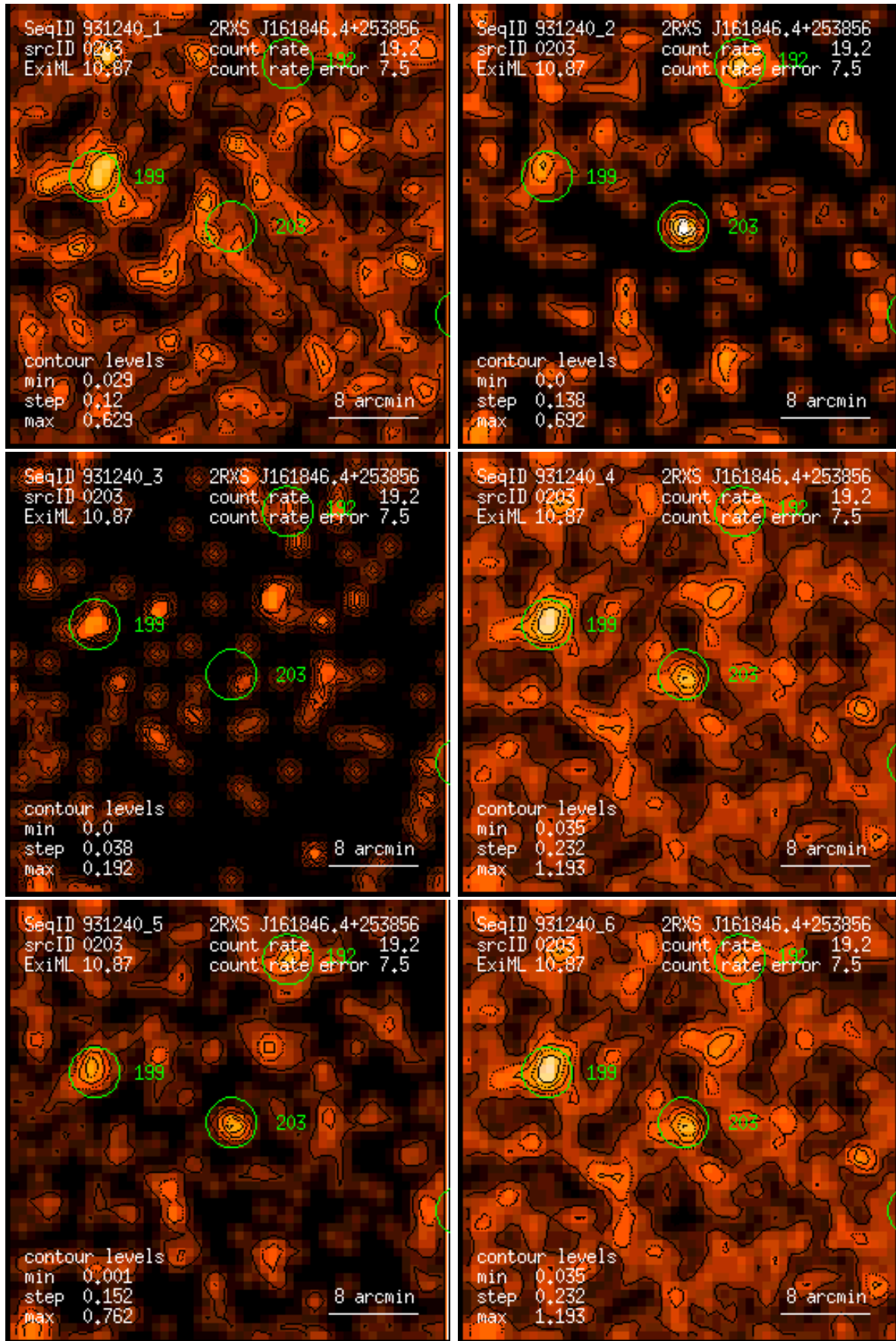
Figure 203: RASS 931240: detection 0203: band rate images, Gaussian filter: (1) PSPC channels 11 – 41, (2) 52 – 90, (3) 91 – 201, (4) 11 – 235, (5) 52 – 201, (6) 11 – 201. Broad band rates in counts/ks. Band rate contour levels in counts/ks/arcmin 2 .
