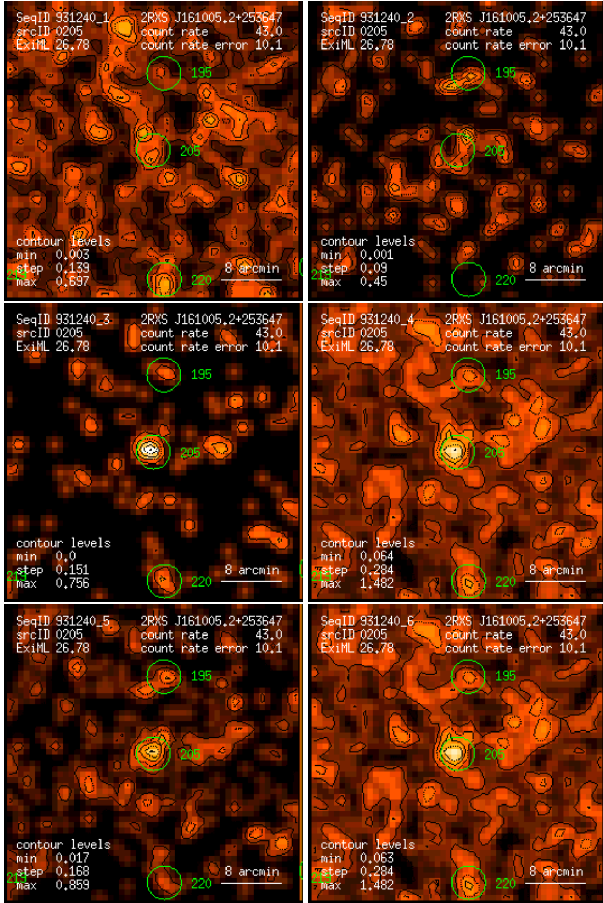
Figure 205: RASS 931240: detection 0205: band rate images, Gaussian filter: (1) PSPC channels 11 – 41, (2) 52 – 90, (3) 91 – 201, (4) 11 – 235, (5) 52 – 201, (6) 11 – 201. Broad band rates in counts/ks. Band rate contour levels in counts/ks/arcmin 2 .
