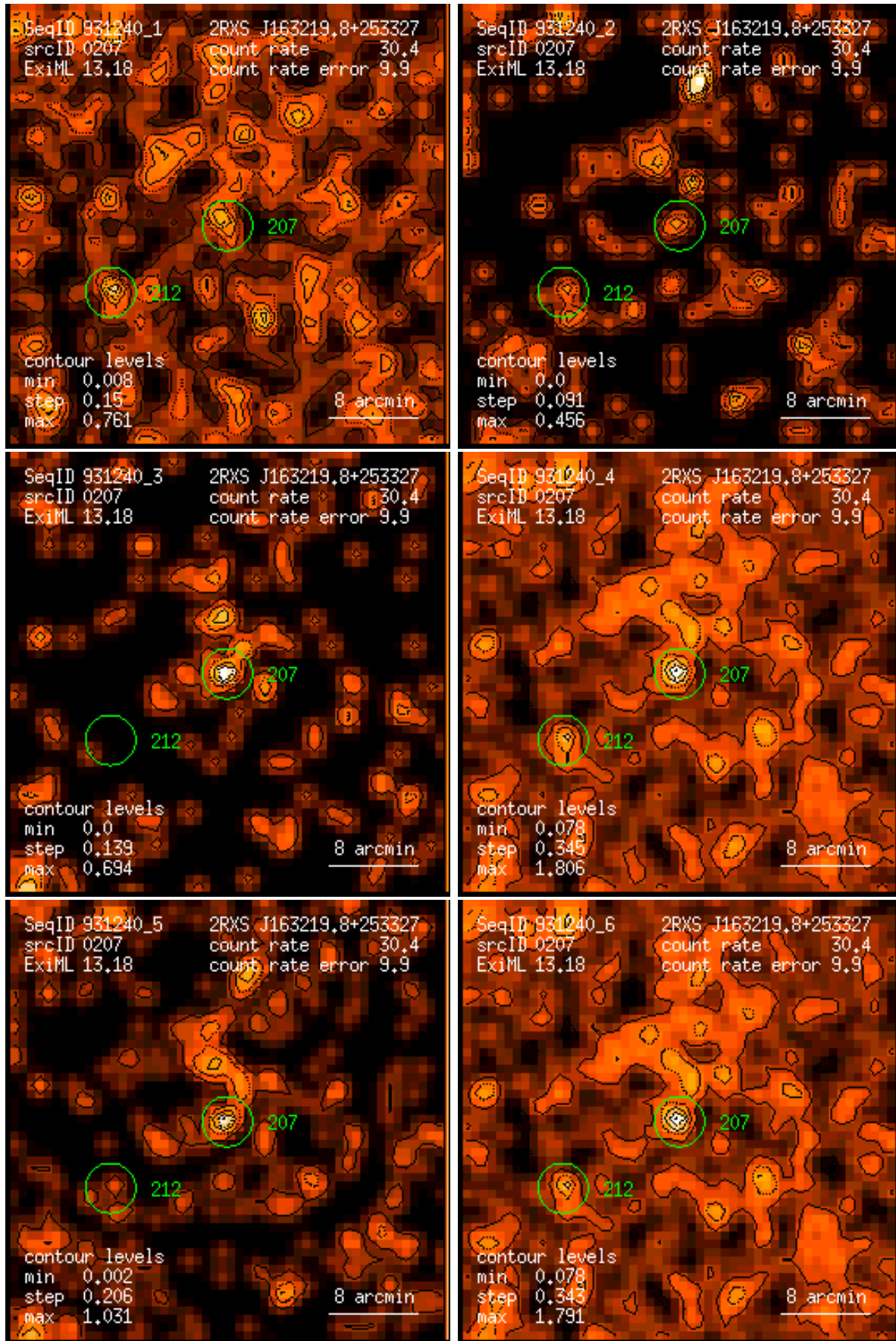
Figure 207: RASS 931240: detection 0207: band rate images, Gaussian filter: (1) PSPC channels 11 – 41, (2) 52 – 90, (3) 91 – 201, (4) 11 – 235, (5) 52 – 201, (6) 11 – 201. Broad band rates in counts/ks. Band rate contour levels in counts/ks/arcmin 2 .
