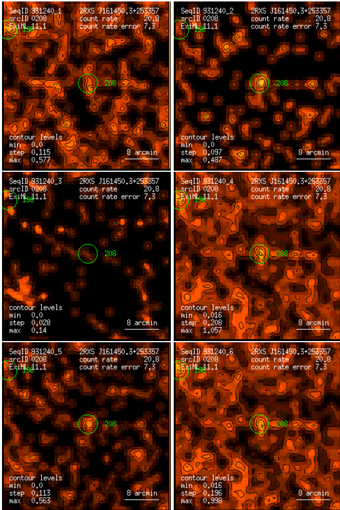
Figure 208: RASS 931240: detection 0208: band rate images, Gaussian filter: (1) PSPC channels 11 – 41, (2) 52 – 90, (3) 91 – 201, (4) 11 – 235, (5) 52 – 201, (6) 11 – 201. Broad band rates in counts/ks. Band rate contour levels in counts/ks/arcmin 2 .
