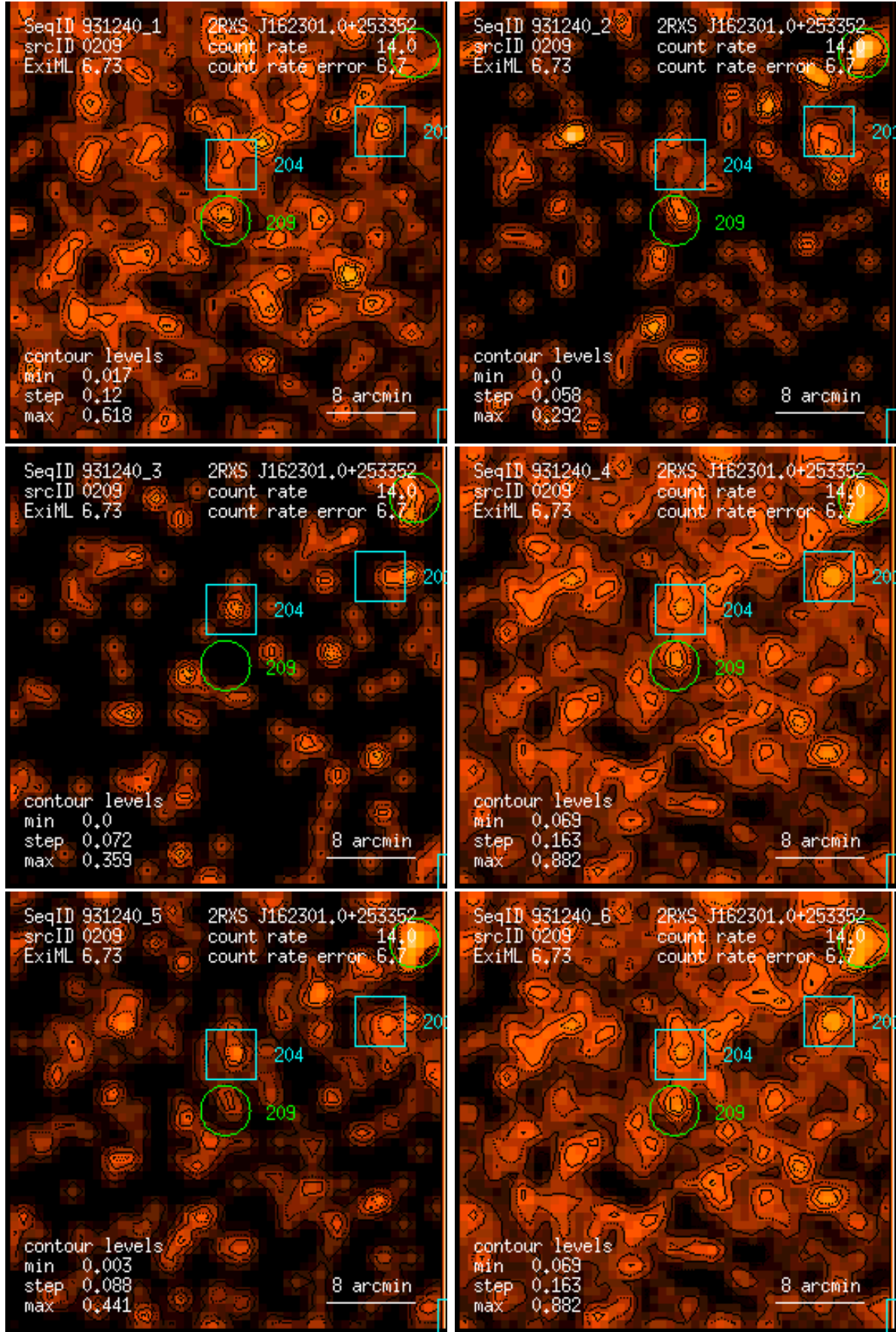
Figure 209: RASS 931240: detection 0209: band rate images, Gaussian filter: (1) PSPC channels 11 – 41, (2) 52 – 90, (3) 91 – 201, (4) 11 – 235, (5) 52 – 201, (6) 11 – 201. Broad band rates in counts/ks. Band rate contour levels in counts/ks/arcmin 2 .
