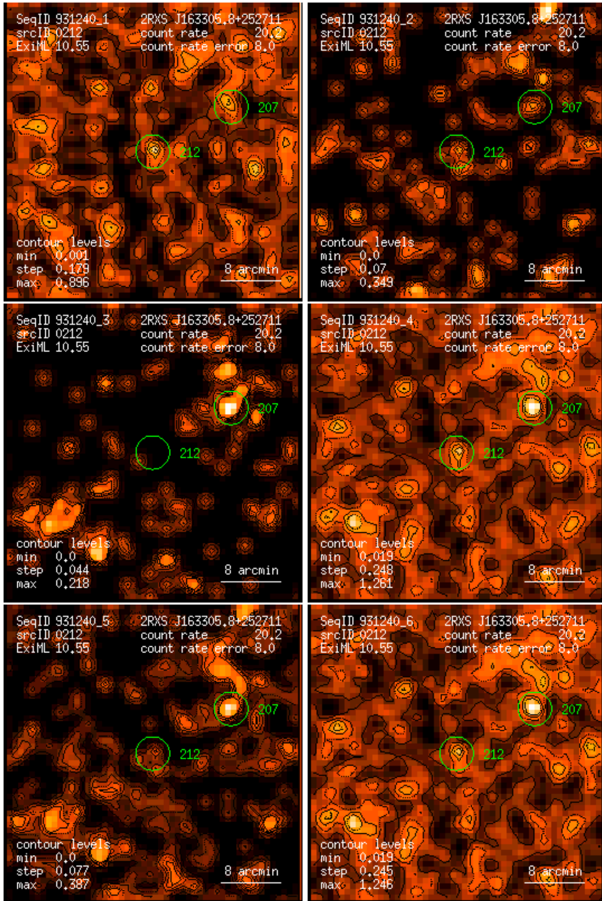
Figure 212: RASS 931240: detection 0212: band rate images, Gaussian filter: (1) PSPC channels 11 – 41, (2) 52 – 90, (3) 91 – 201, (4) 11 – 235, (5) 52 – 201, (6) 11 – 201. Broad band rates in counts/ks. Band rate contour levels in counts/ks/arcmin 2 .
