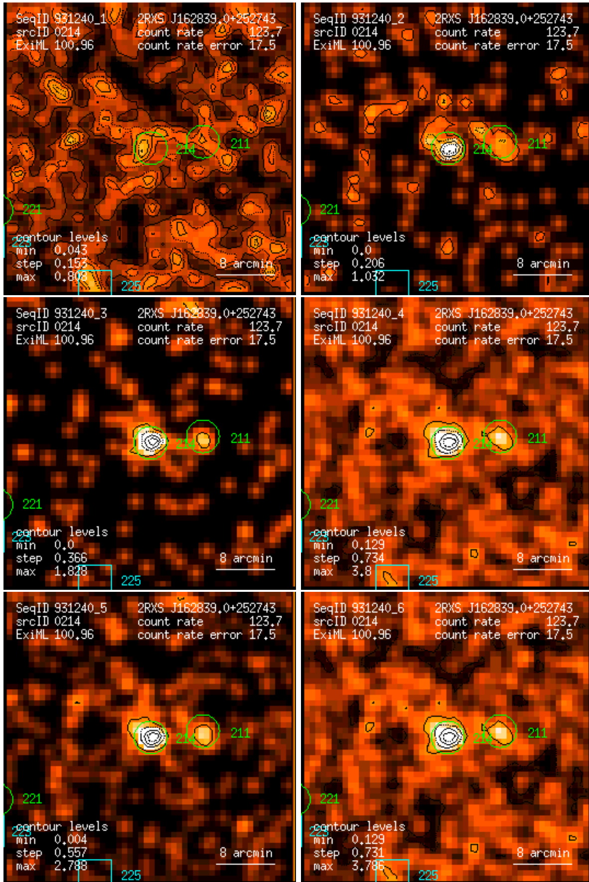
Figure 214: RASS 931240: detection 0214: band rate images, Gaussian filter: (1) PSPC channels 11 – 41, (2) 52 – 90, (3) 91 – 201, (4) 11 – 235, (5) 52 – 201, (6) 11 – 201. Broad band rates in counts/ks. Band rate contour levels in counts/ks/arcmin 2 .
