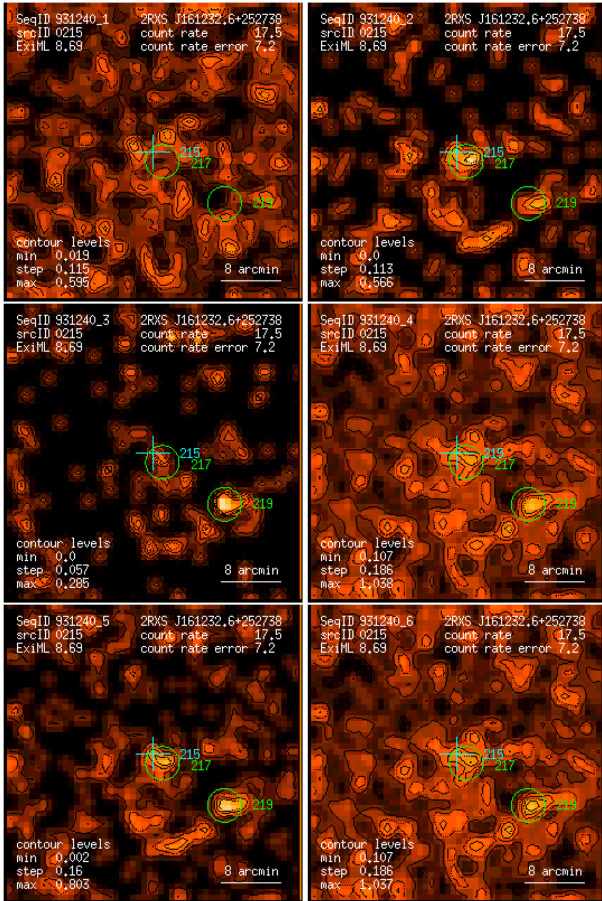
Figure 215: RASS 931240: detection 0215: band rate images, Gaussian filter: (1) PSPC channels 11 – 41, (2) 52 – 90, (3) 91 – 201, (4) 11 – 235, (5) 52 – 201, (6) 11 – 201. Broad band rates in counts/ks. Band rate contour levels in counts/ks/arcmin 2 .
