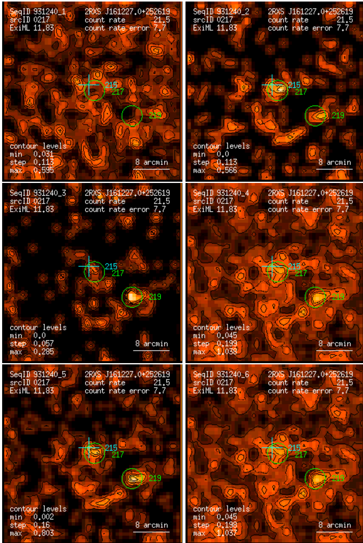
Figure 217: RASS 931240: detection 0217: band rate images, Gaussian filter: (1) PSPC channels 11 – 41, (2) 52 – 90, (3) 91 – 201, (4) 11 – 235, (5) 52 – 201, (6) 11 – 201. Broad band rates in counts/ks. Band rate contour levels in counts/ks/arcmin 2 .
