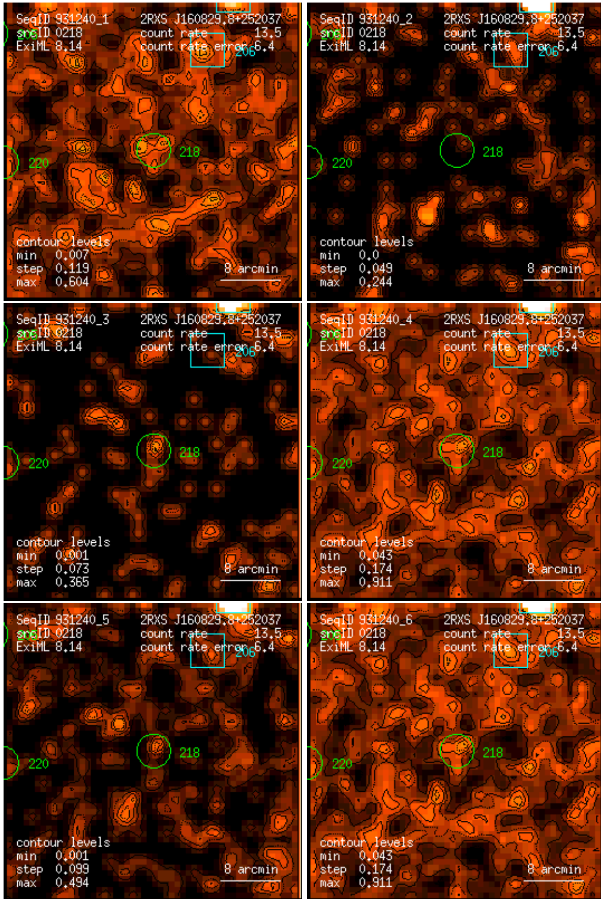
Figure 218: RASS 931240: detection 0218: band rate images, Gaussian filter: (1) PSPC channels 11 – 41, (2) 52 – 90, (3) 91 – 201, (4) 11 – 235, (5) 52 – 201, (6) 11 – 201. Broad band rates in counts/ks. Band rate contour levels in counts/ks/arcmin 2 .
