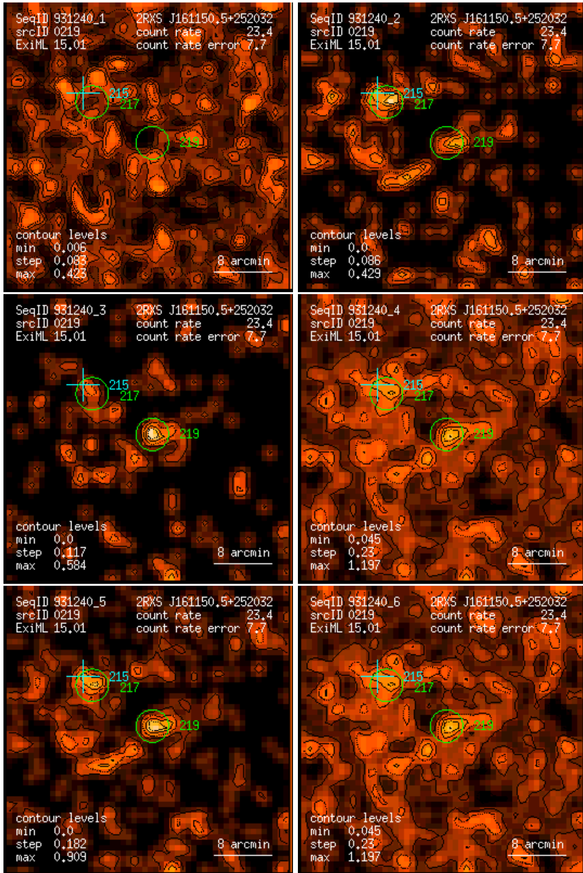
Figure 219: RASS 931240: detection 0219: band rate images, Gaussian filter: (1) PSPC channels 11 – 41, (2) 52 – 90, (3) 91 – 201, (4) 11 – 235, (5) 52 – 201, (6) 11 – 201. Broad band rates in counts/ks. Band rate contour levels in counts/ks/arcmin 2 .
