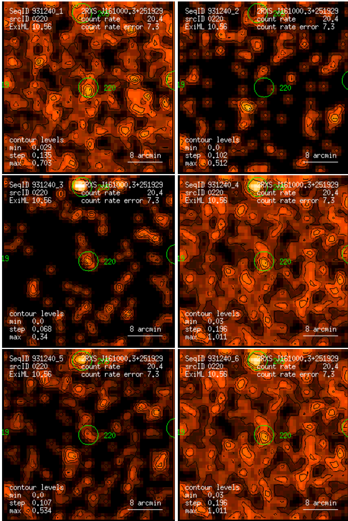
Figure 220: RASS 931240: detection 0220: band rate images, Gaussian filter: (1) PSPC channels 11 – 41, (2) 52 – 90, (3) 91 – 201, (4) 11 – 235, (5) 52 – 201, (6) 11 – 201. Broad band rates in counts/ks. Band rate contour levels in counts/ks/arcmin 2 .
