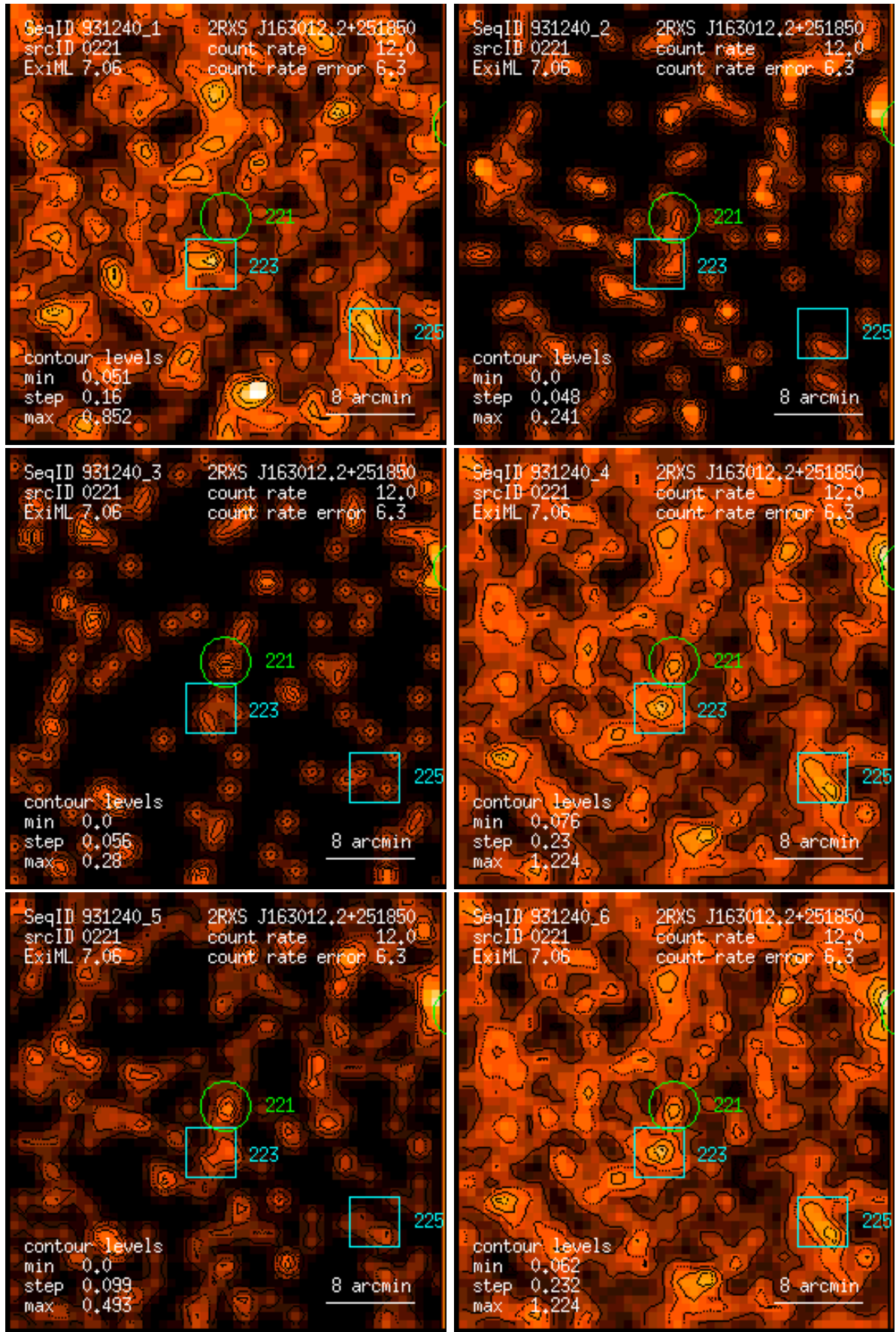
Figure 221: RASS 931240: detection 0221: band rate images, Gaussian filter: (1) PSPC channels 11 – 41, (2) 52 – 90, (3) 91 – 201, (4) 11 – 235, (5) 52 – 201, (6) 11 – 201. Broad band rates in counts/ks. Band rate contour levels in counts/ks/arcmin 2 .
