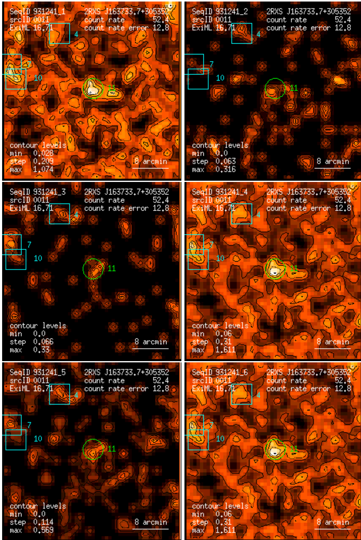
Figure 11: RASS 931241: detection 0011: band rate images, Gaussian filter: (1) PSPC channels 11 – 41, (2) 52 – 90, (3) 91 – 201, (4) 11 – 235, (5) 52 – 201, (6) 11 – 201. Broad band rates in counts/ks. Band rate contour levels in counts/ks/arcmin 2 .
