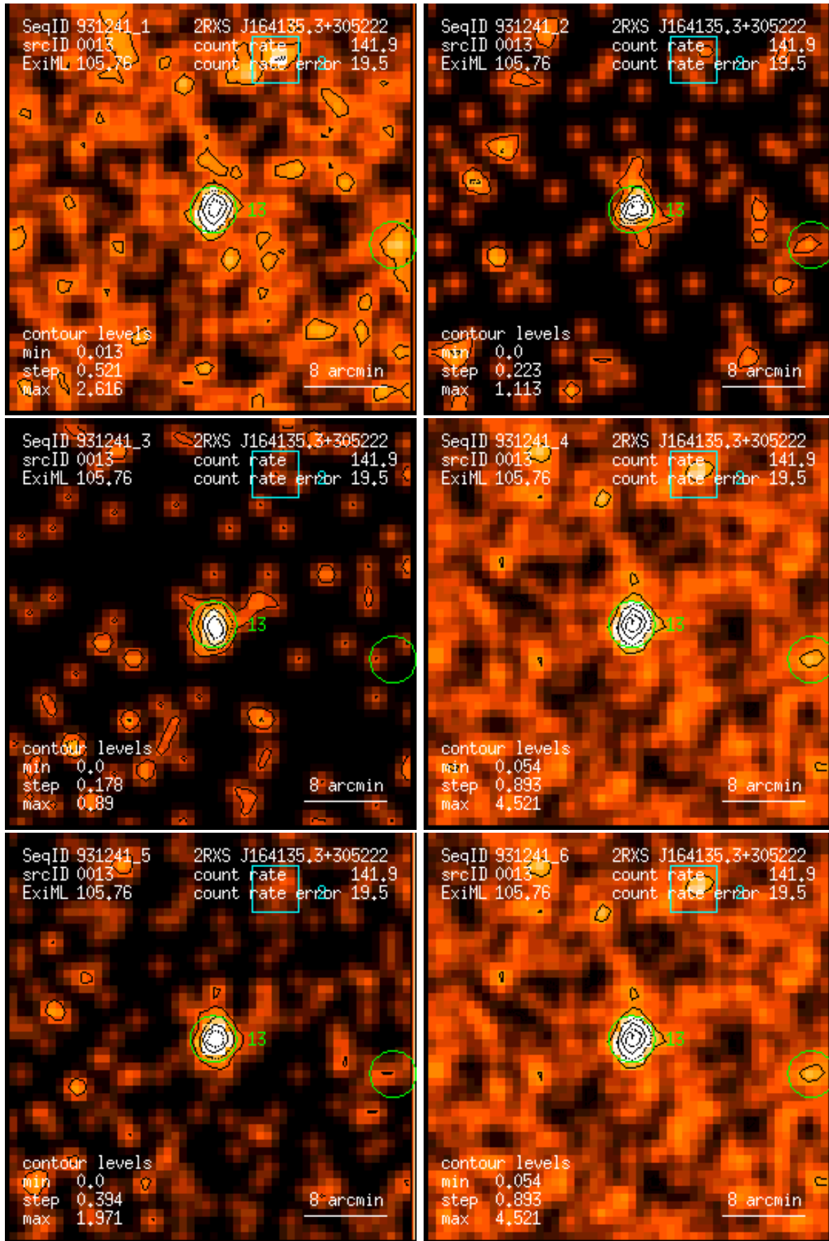
Figure 13: RASS 931241: detection 0013: band rate images, Gaussian filter: (1) PSPC channels 11 – 41, (2) 52 – 90, (3) 91 – 201, (4) 11 – 235, (5) 52 – 201, (6) 11 – 201. Broad band rates in counts/ks. Band rate contour levels in counts/ks/arcmin 2 .
