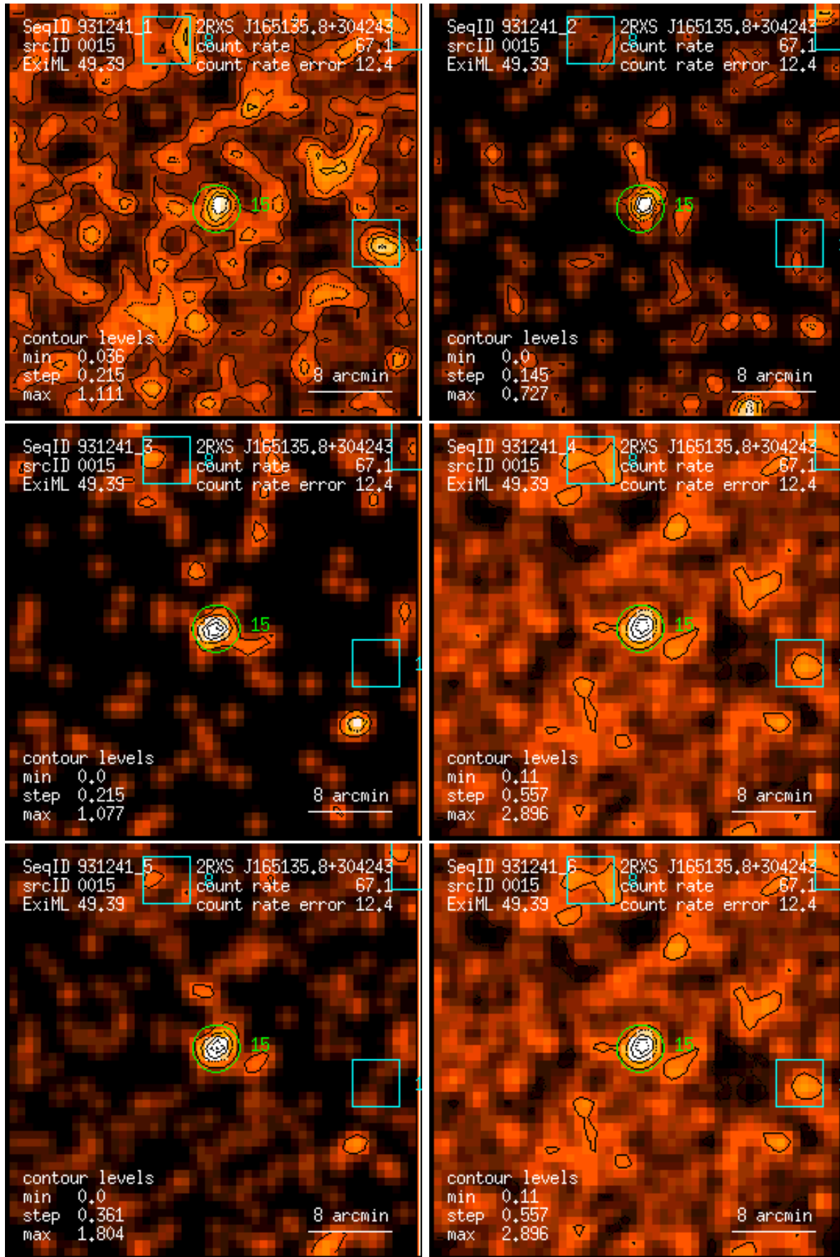
Figure 15: RASS 931241: detection 0015: band rate images, Gaussian filter: (1) PSPC channels 11 – 41, (2) 52 – 90, (3) 91 – 201, (4) 11 – 235, (5) 52 – 201, (6) 11 – 201. Broad band rates in counts/ks. Band rate contour levels in counts/ks/arcmin 2 .
