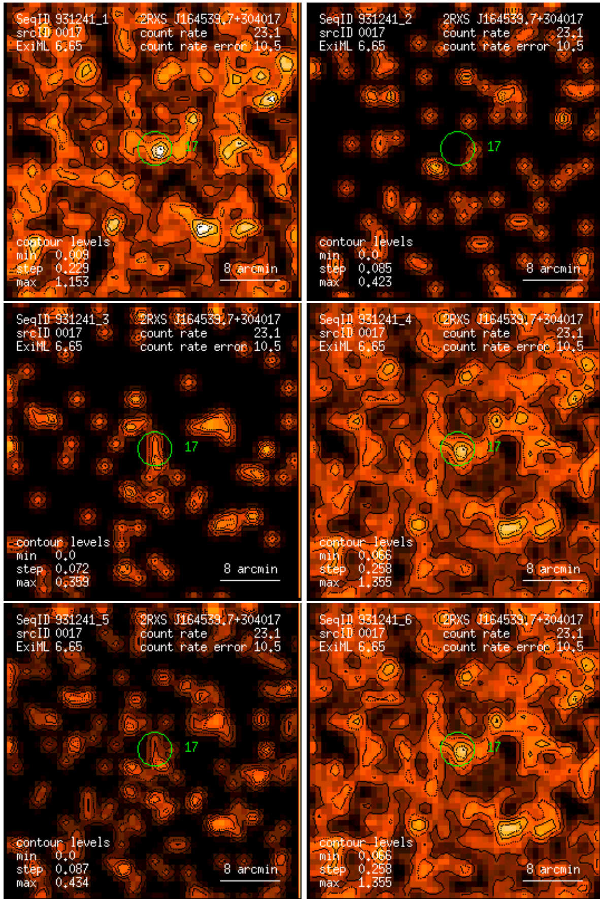
Figure 17: RASS 931241: detection 0017: band rate images, Gaussian filter: (1) PSPC channels 11 – 41, (2) 52 – 90, (3) 91 – 201, (4) 11 – 235, (5) 52 – 201, (6) 11 – 201. Broad band rates in counts/ks. Band rate contour levels in counts/ks/arcmin 2 .
