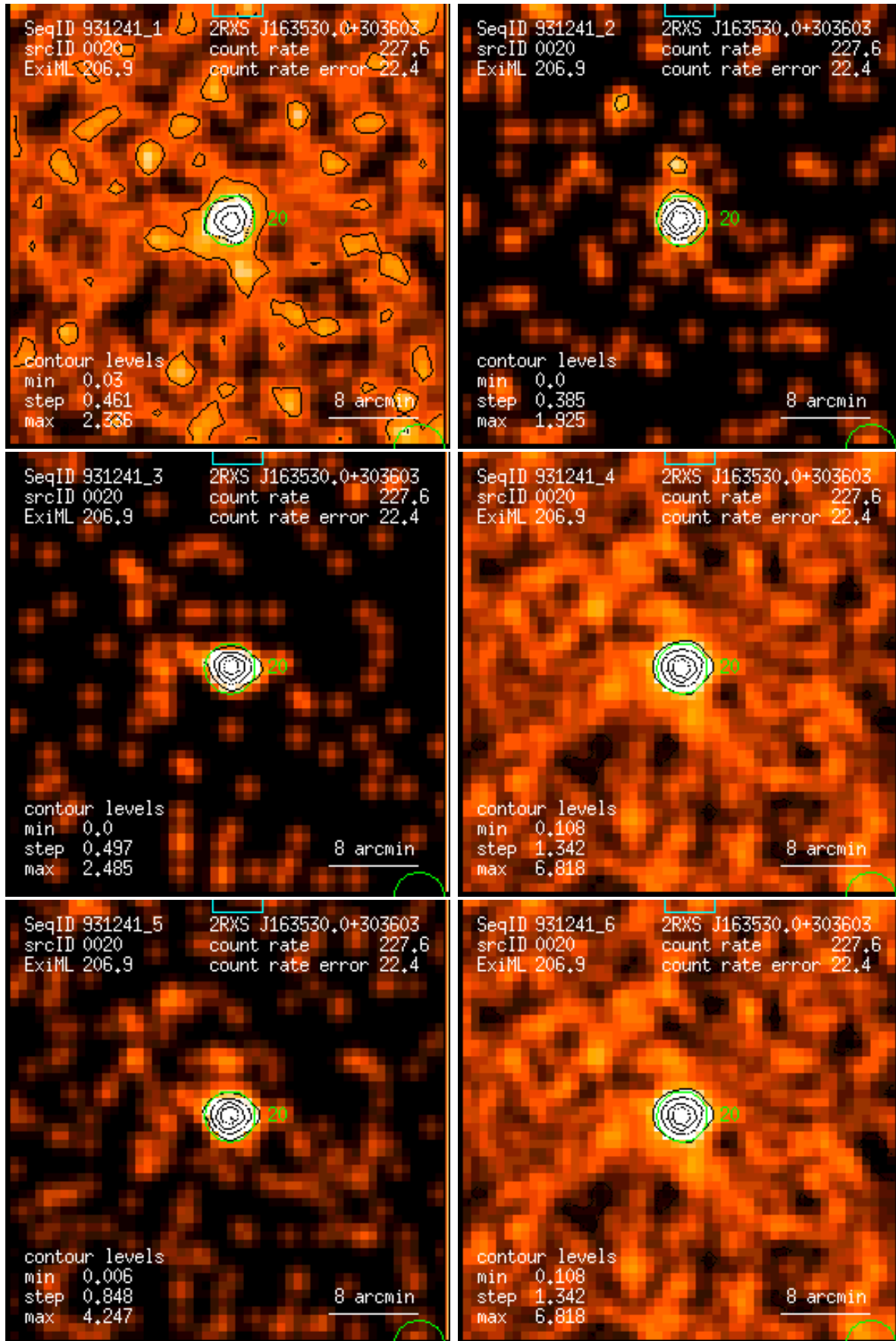
Figure 20: RASS 931241: detection 0020: band rate images, Gaussian filter: (1) PSPC channels 11 – 41, (2) 52 – 90, (3) 91 – 201, (4) 11 – 235, (5) 52 – 201, (6) 11 – 201. Broad band rates in counts/ks. Band rate contour levels in counts/ks/arcmin 2 .
