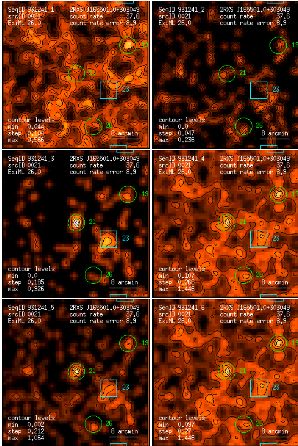
Figure 21: RASS 931241: detection 0021: band rate images, Gaussian filter: (1) PSPC channels 11 – 41, (2) 52 – 90, (3) 91 – 201, (4) 11 – 235, (5) 52 – 201, (6) 11 – 201. Broad band rates in counts/ks. Band rate contour levels in counts/ks/arcmin 2 .
