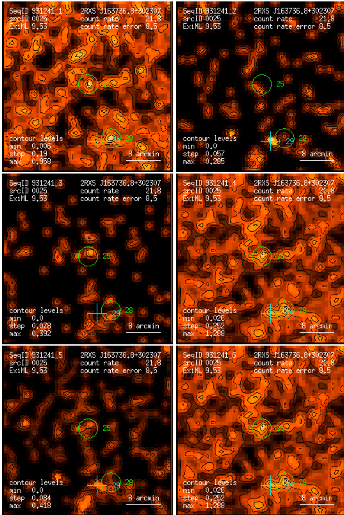
Figure 25: RASS 931241: detection 0025: band rate images, Gaussian filter: (1) PSPC channels 11 – 41, (2) 52 – 90, (3) 91 – 201, (4) 11 – 235, (5) 52 – 201, (6) 11 – 201. Broad band rates in counts/ks. Band rate contour levels in counts/ks/arcmin 2 .
