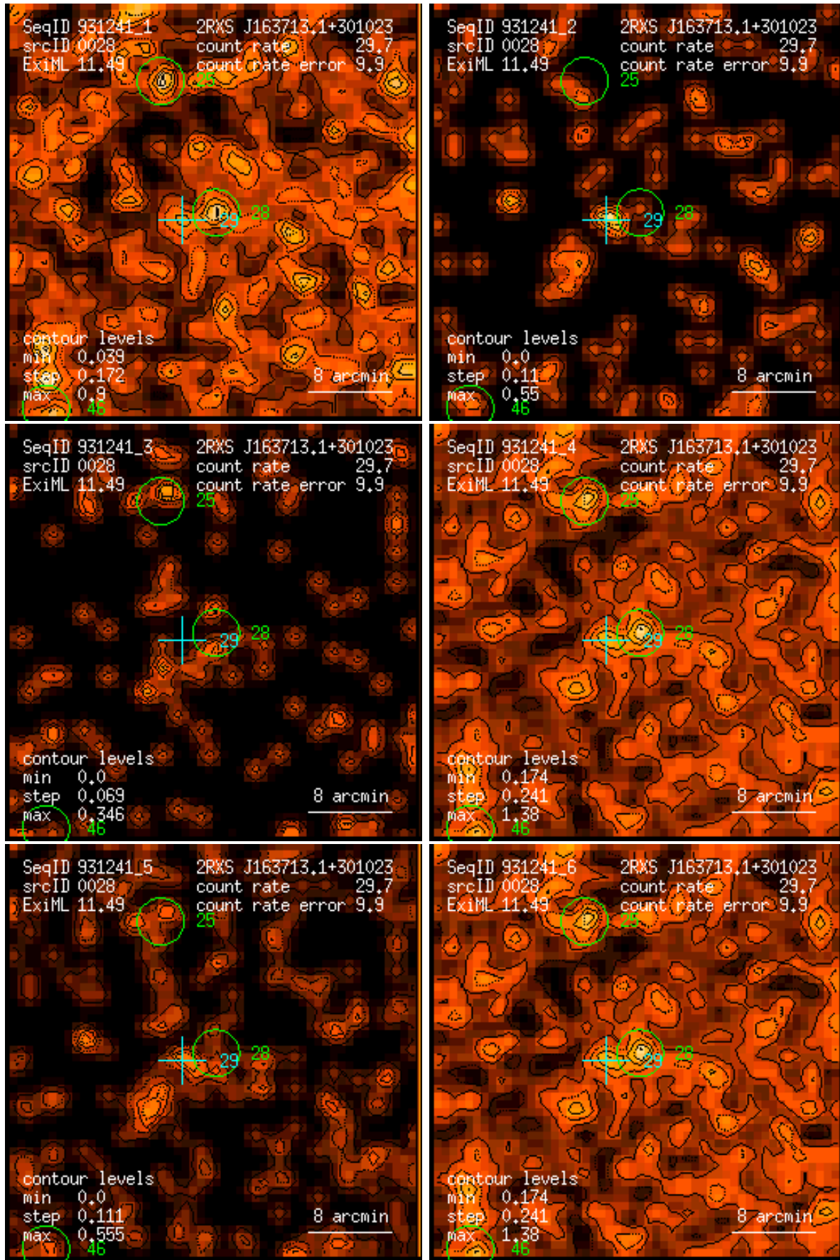
Figure 28: RASS 931241: detection 0028: band rate images, Gaussian filter: (1) PSPC channels 11 – 41, (2) 52 – 90, (3) 91 – 201, (4) 11 – 235, (5) 52 – 201, (6) 11 – 201. Broad band rates in counts/ks. Band rate contour levels in counts/ks/arcmin 2 .
