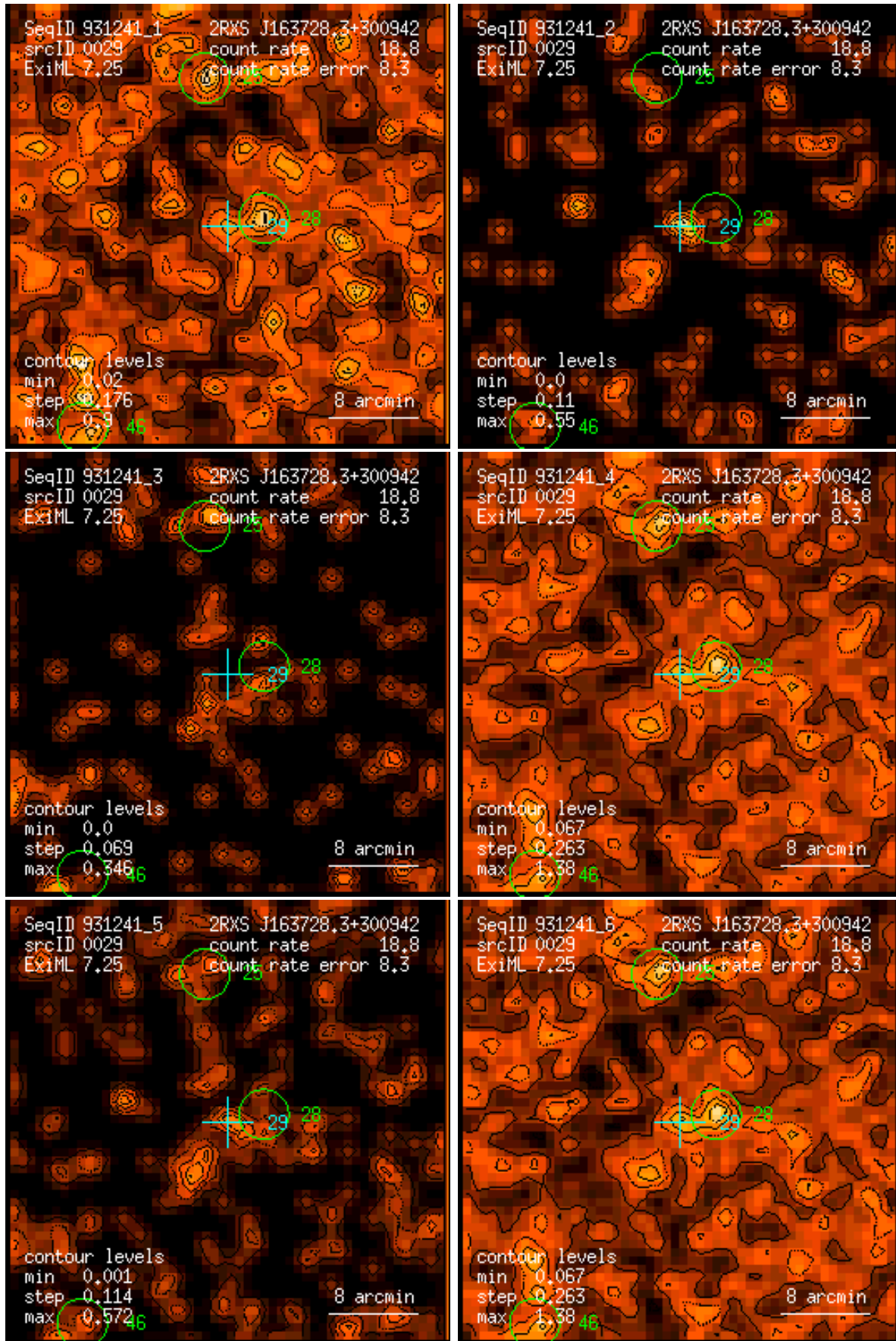
Figure 29: RASS 931241: detection 0029: band rate images, Gaussian filter: (1) PSPC channels 11 – 41, (2) 52 – 90, (3) 91 – 201, (4) 11 – 235, (5) 52 – 201, (6) 11 – 201. Broad band rates in counts/ks. Band rate contour levels in counts/ks/arcmin 2 .
