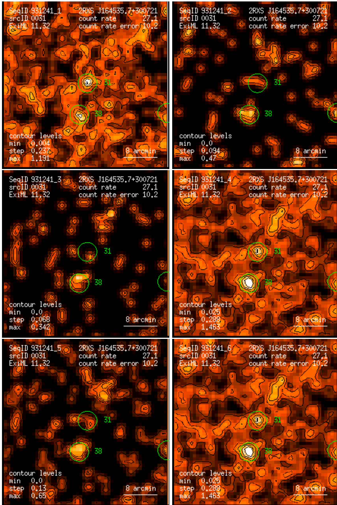
Figure 31: RASS 931241: detection 0031: band rate images, Gaussian filter: (1) PSPC channels 11 – 41, (2) 52 – 90, (3) 91 – 201, (4) 11 – 235, (5) 52 – 201, (6) 11 – 201. Broad band rates in counts/ks. Band rate contour levels in counts/ks/arcmin 2 .
