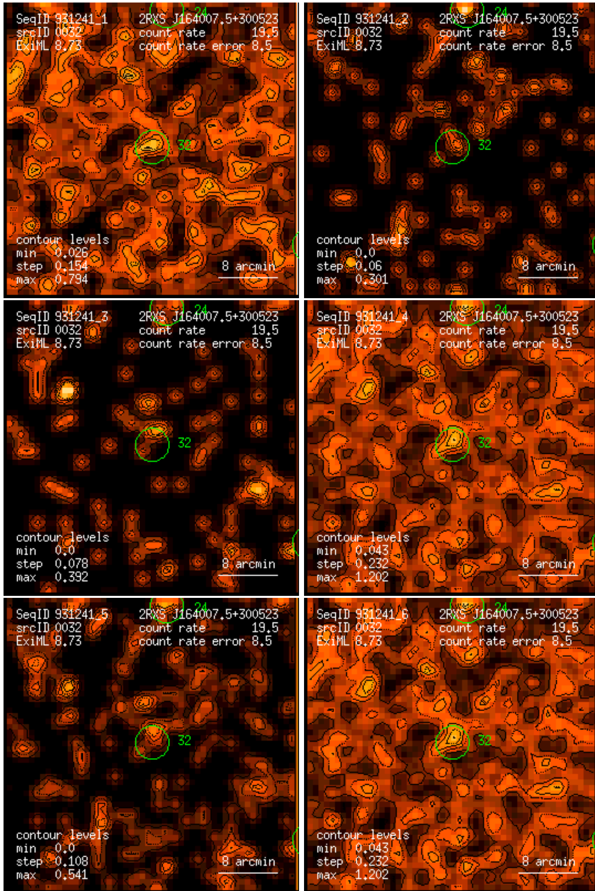
Figure 32: RASS 931241: detection 0032: band rate images, Gaussian filter: (1) PSPC channels 11 – 41, (2) 52 – 90, (3) 91 – 201, (4) 11 – 235, (5) 52 – 201, (6) 11 – 201. Broad band rates in counts/ks. Band rate contour levels in counts/ks/arcmin 2 .
