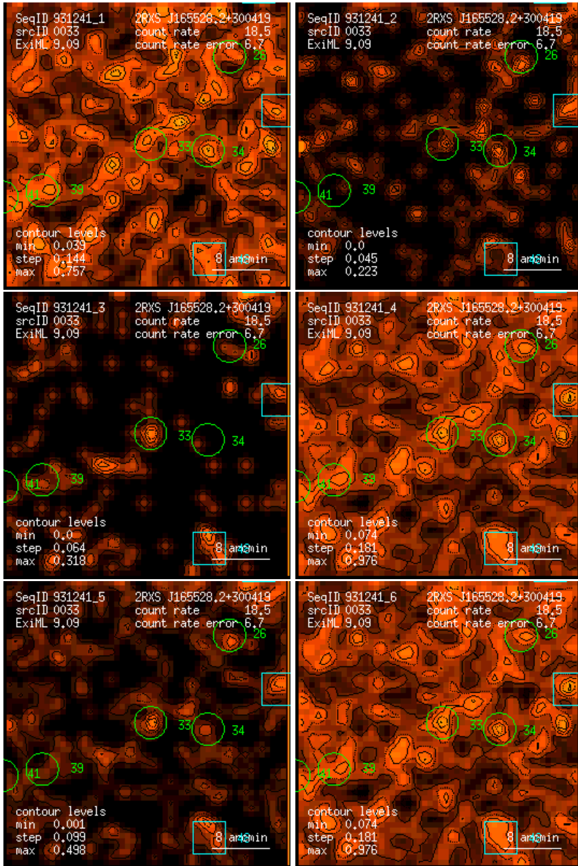
Figure 33: RASS 931241: detection 0033: band rate images, Gaussian filter: (1) PSPC channels 11 – 41, (2) 52 – 90, (3) 91 – 201, (4) 11 – 235, (5) 52 – 201, (6) 11 – 201. Broad band rates in counts/ks. Band rate contour levels in counts/ks/arcmin 2 .
