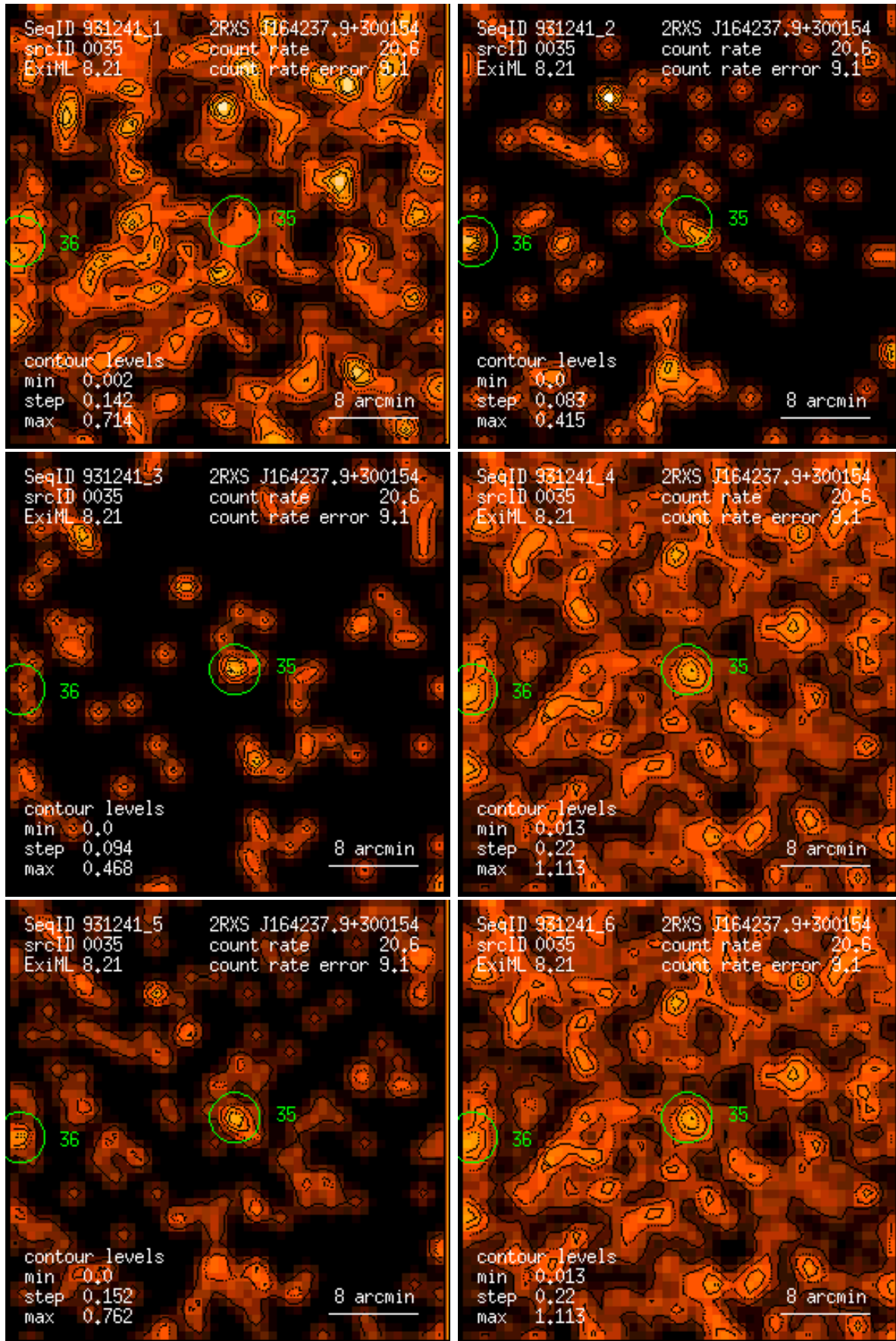
Figure 35: RASS 931241: detection 0035: band rate images, Gaussian filter: (1) PSPC channels 11 – 41, (2) 52 – 90, (3) 91 – 201, (4) 11 – 235, (5) 52 – 201, (6) 11 – 201. Broad band rates in counts/ks. Band rate contour levels in counts/ks/arcmin 2 .
