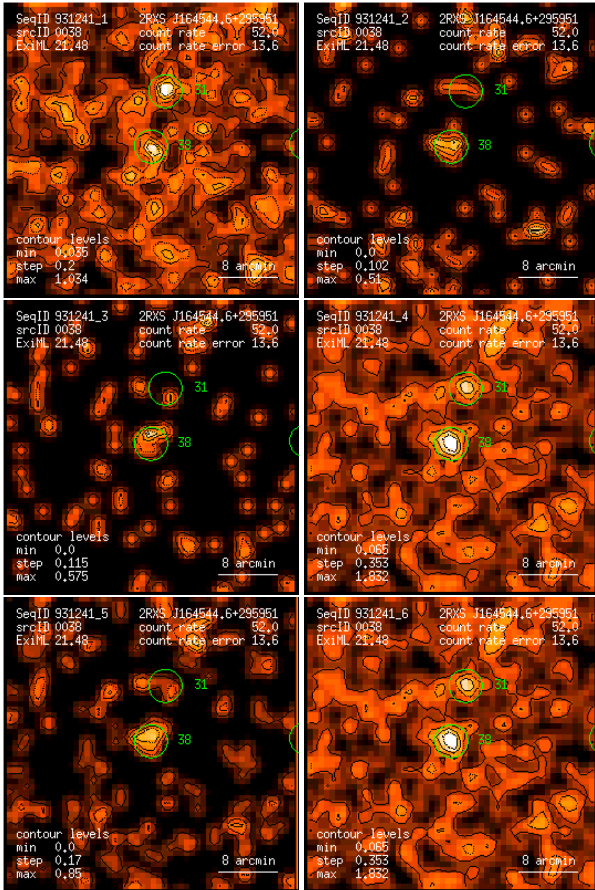
Figure 38: RASS 931241: detection 0038: band rate images, Gaussian filter: (1) PSPC channels 11 – 41, (2) 52 – 90, (3) 91 – 201, (4) 11 – 235, (5) 52 – 201, (6) 11 – 201. Broad band rates in counts/ks. Band rate contour levels in counts/ks/arcmin 2 .
