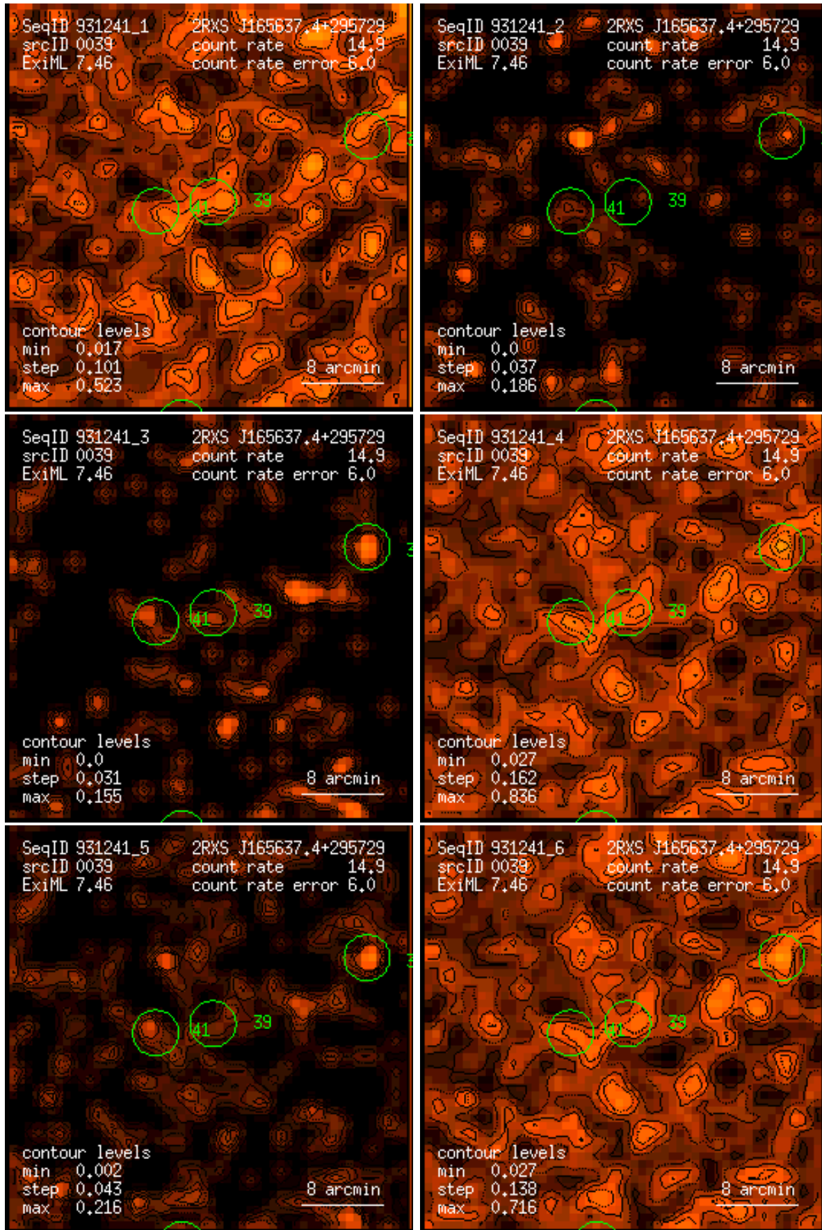
Figure 39: RASS 931241: detection 0039: band rate images, Gaussian filter: (1) PSPC channels 11 – 41, (2) 52 – 90, (3) 91 – 201, (4) 11 – 235, (5) 52 – 201, (6) 11 – 201. Broad band rates in counts/ks. Band rate contour levels in counts/ks/arcmin 2 .
