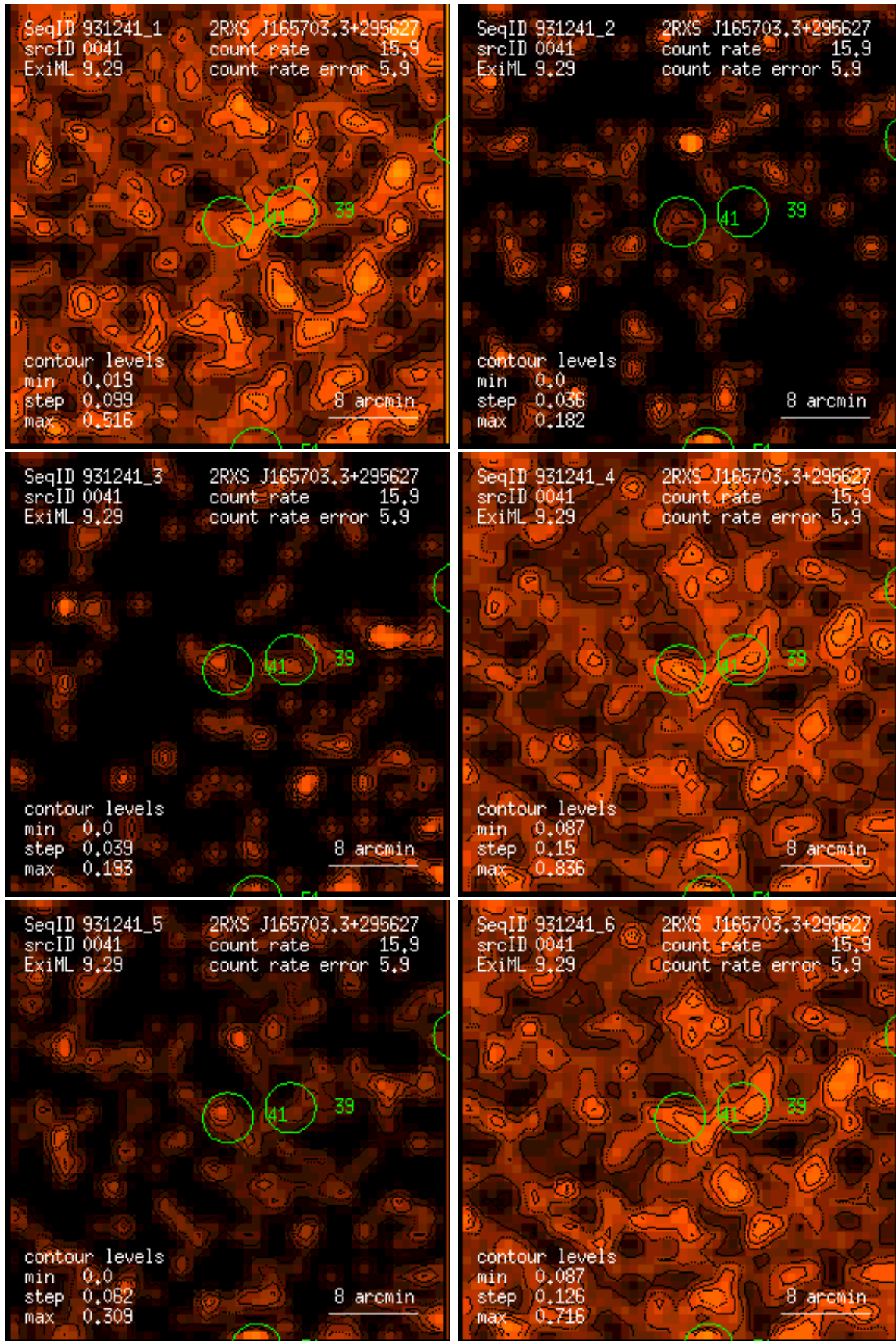
Figure 41: RASS 931241: detection 0041: band rate images, Gaussian filter: (1) PSPC channels 11 – 41, (2) 52 – 90, (3) 91 – 201, (4) 11 – 235, (5) 52 – 201, (6) 11 – 201. Broad band rates in counts/ks. Band rate contour levels in counts/ks/arcmin 2 .
