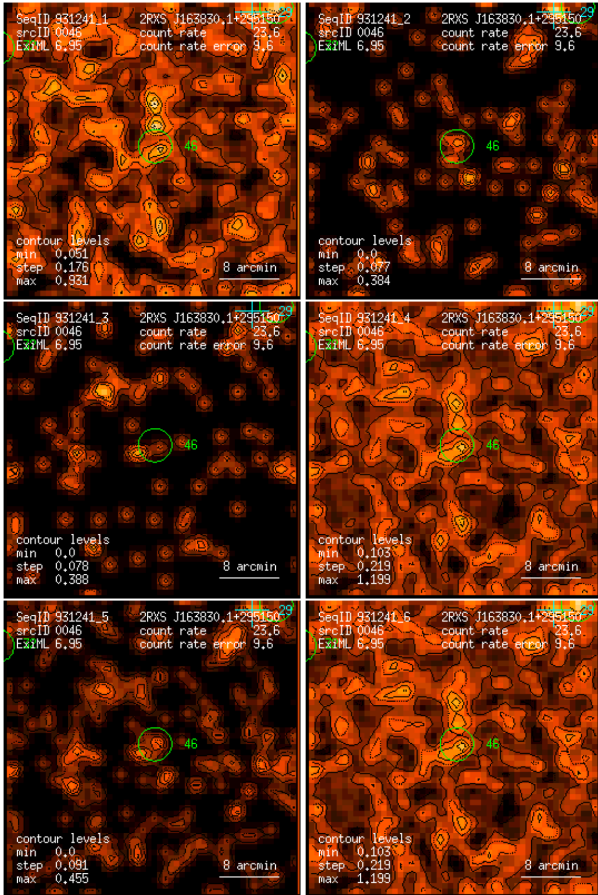
Figure 46: RASS 931241: detection 0046: band rate images, Gaussian filter: (1) PSPC channels 11 – 41, (2) 52 – 90, (3) 91 – 201, (4) 11 – 235, (5) 52 – 201, (6) 11 – 201. Broad band rates in counts/ks. Band rate contour levels in counts/ks/arcmin 2 .
