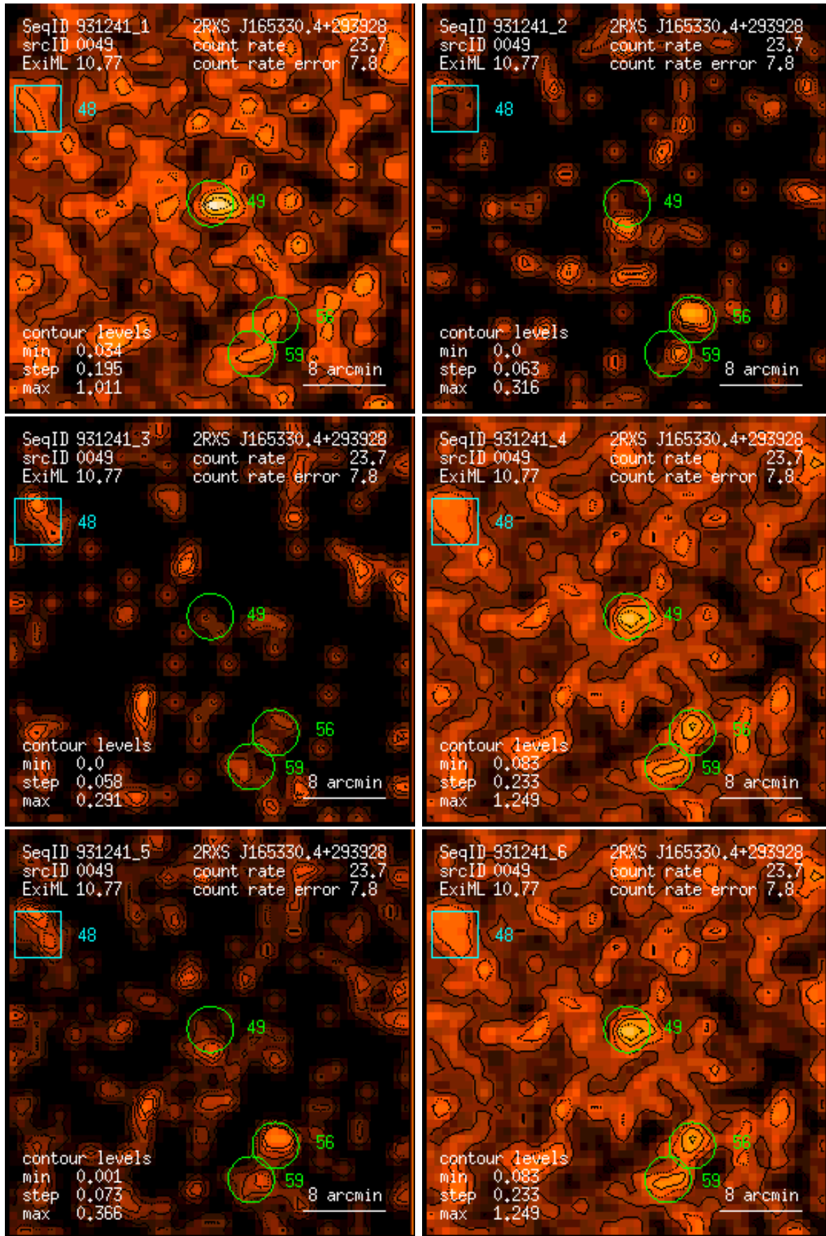
Figure 49: RASS 931241: detection 0049: band rate images, Gaussian filter: (1) PSPC channels 11 – 41, (2) 52 – 90, (3) 91 – 201, (4) 11 – 235, (5) 52 – 201, (6) 11 – 201. Broad band rates in counts/ks. Band rate contour levels in counts/ks/arcmin 2 .
