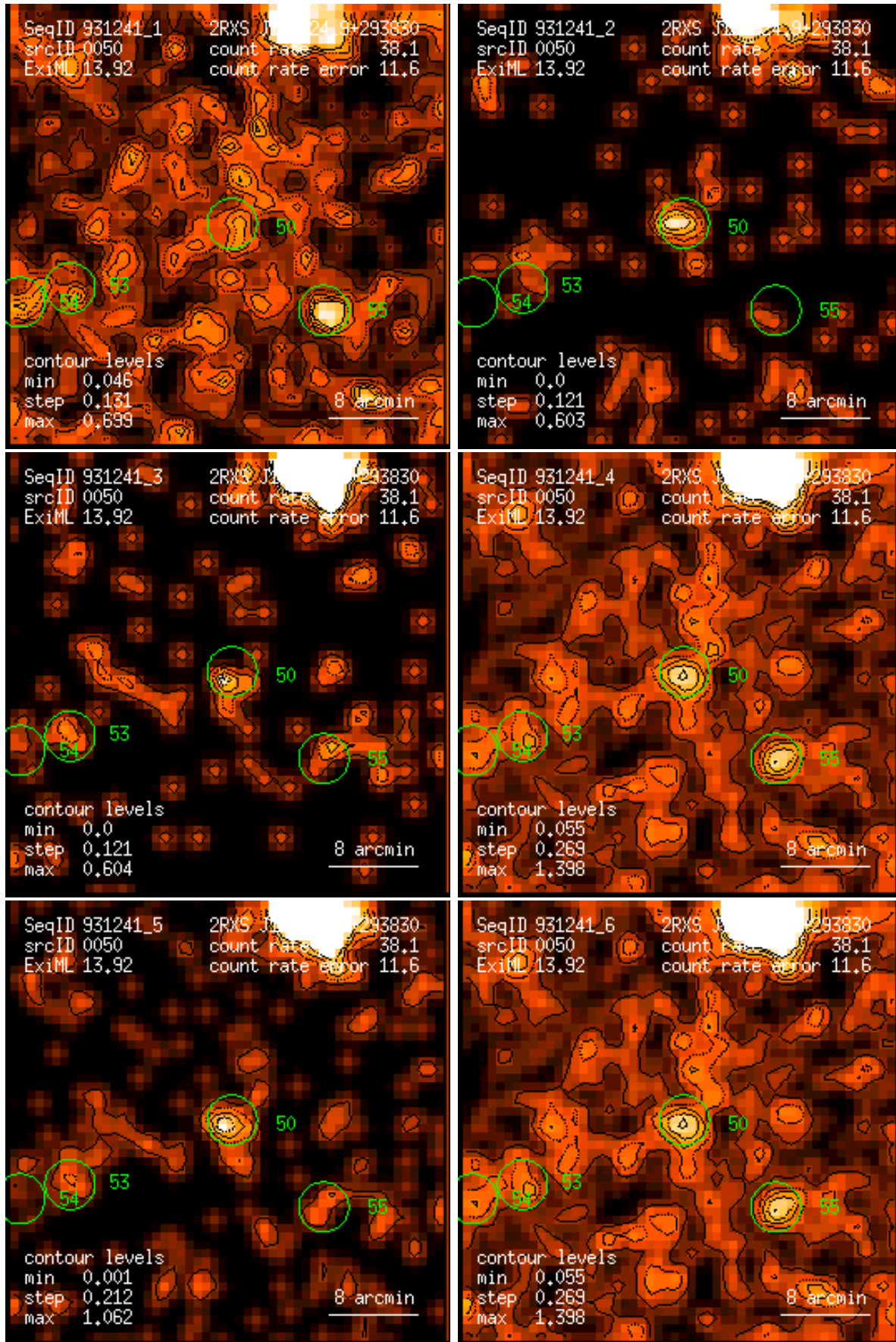
Figure 50: RASS 931241: detection 0050: band rate images, Gaussian filter: (1) PSPC channels 11 – 41, (2) 52 – 90, (3) 91 – 201, (4) 11 – 235, (5) 52 – 201, (6) 11 – 201. Broad band rates in counts/ks. Band rate contour levels in counts/ks/arcmin 2 .
