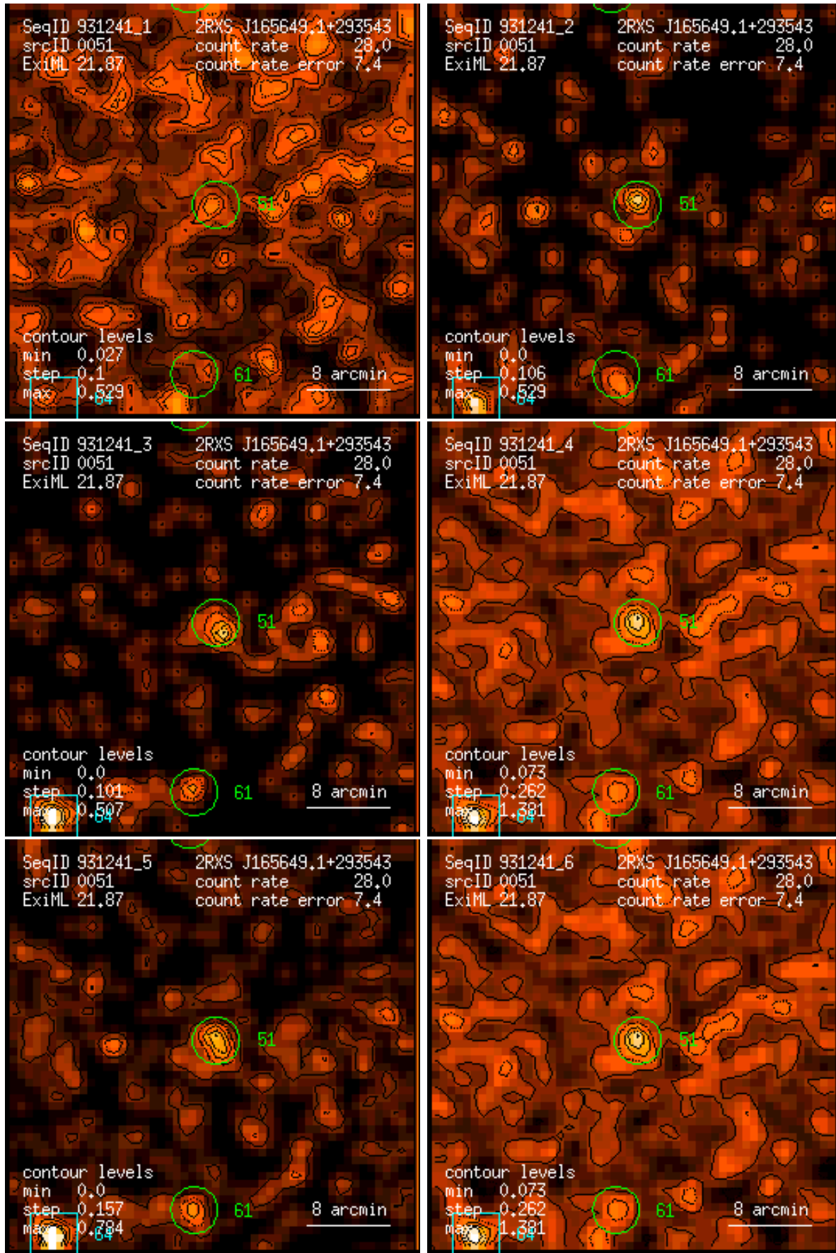
Figure 51: RASS 931241: detection 0051: band rate images, Gaussian filter: (1) PSPC channels 11 – 41, (2) 52 – 90, (3) 91 – 201, (4) 11 – 235, (5) 52 – 201, (6) 11 – 201. Broad band rates in counts/ks. Band rate contour levels in counts/ks/arcmin 2 .
